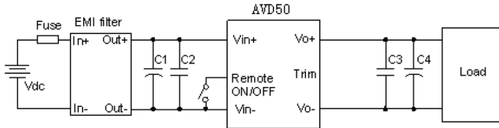
Figure 15 Typical application
