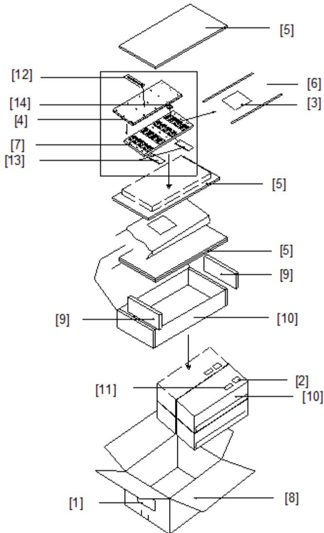
Figure 20 Package disassembly
