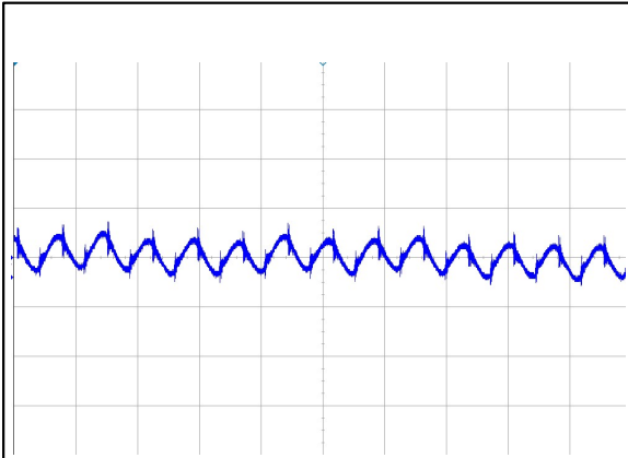
Figure 1: AVE350B-48S28 Input Reflected Ripple Current Waveform Ch 1: I in (5 \mu S/div, 50mA/div)
