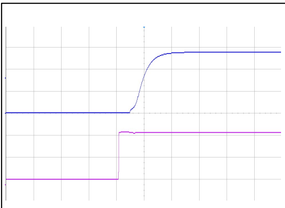
Figure 3: AVE350B-48S28 Output Voltage Startup Characteristic (20mS/div) Ch 1: V in (10V/div) Ch 2: V o (20V/div)
