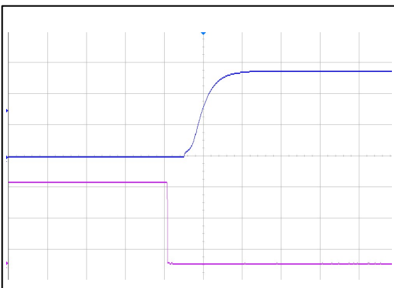
Figure 5: AVE350B-48S28 Remote ON Waveform (20mS/div) Ch 1: Remote ON (10V/div) Ch 2: V o (2V/div)
