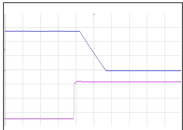
Figure 6: AVE350B-48S28 Remote OFF Waveform (1mS/div) Ch 1: Remote OFF (10V/div) CH3: V o (2V/div)
