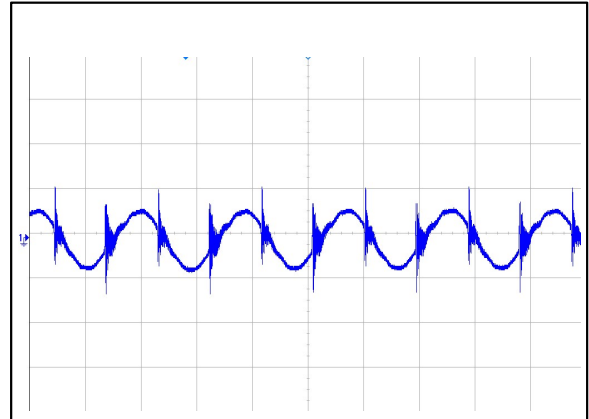
Figure 2: AVE350B-48S28 Ripple and Noise Measurement Ch 1: V o (2 \mu S/div, 50mV/div)
