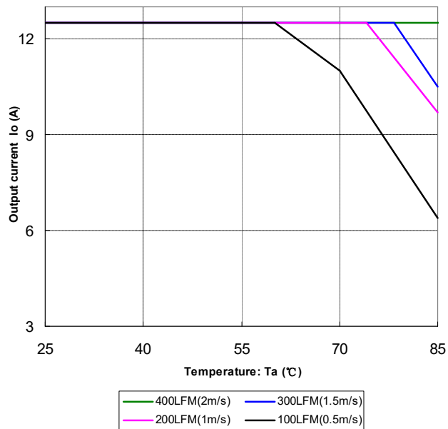
Figure 13 Output power derating, 48Vin
