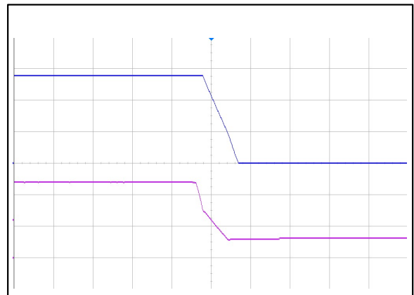
Figure 4: AVE350B-48S28 Turn Off Characteristic (5mS/div) Ch 1: V in (10V/div) Ch 2: V o (20V/div)
