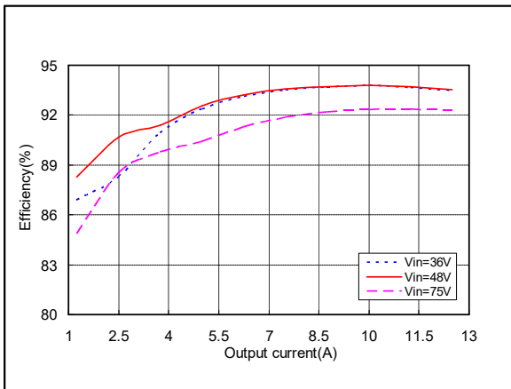
Figure 9: AVE350B-48S28 Efficiency Curves V_o=28Vdc
