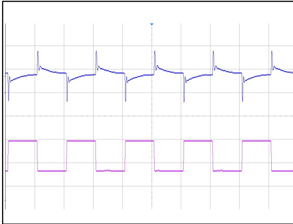
Figure 7: AVE350B-48S28 Transient Response (5mS/div) 25%-50%-25% load change, 0.1A/uS slew rate, Ch 1: Vo (200mV/div) Ch 2: Io (2.5A/div)
