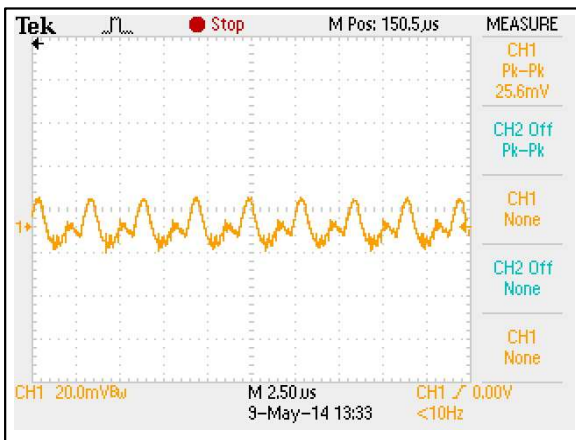
Figure 93: AEE02C36-L Ripple and Noise Measurement Vin = 48Vdc Load: Io = 2.67A Ch 1: Vo
