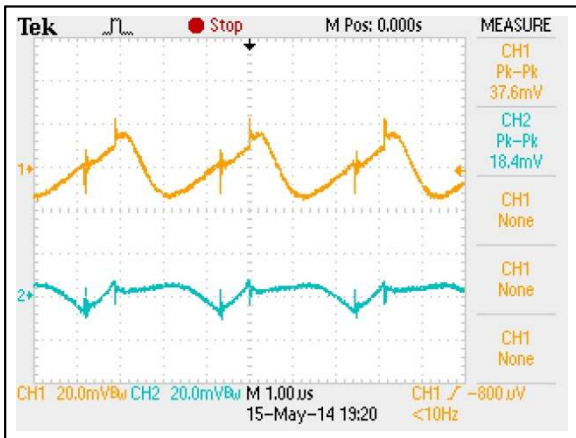
Figure 48: AEE01BB18-L Ripple and Noise Measurement Vin = 24Vdc Load: Io = ±1.67A Ch 1: Vo1 Ch 1: Vo2
