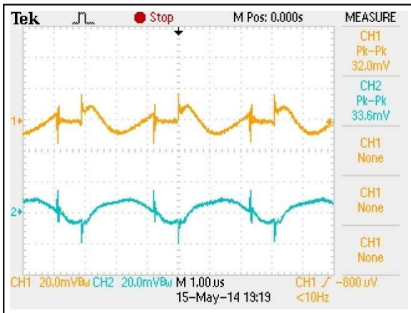
Figure 57: AEE01CC18-L Ripple and Noise Measurement Vin = 48Vdc Load: Io = ±1.33A Ch 1: Vo1 Ch 1: Vo2
