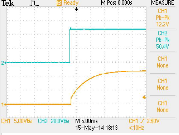
Figure 114: AEE01BB36-L Output Voltage Startup Characteristic by Vin Vin = 48Vdc Load: Io = ±1.67A Ch 1: Vo Ch 2: Vin
