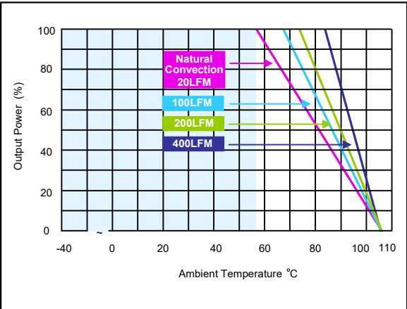
Figure 106: AEE01H36-L Derating Curves (without heatsink) Vin = 48Vdc Load: Io = 0 to 1.67A
