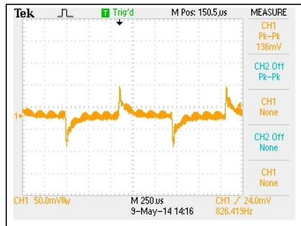
Figure 94: AEE02C36-L Transient Response Vin = 48Vdc Load: Io = 100% to 75% load change Ch 1: Vo
