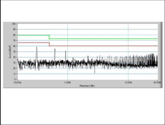
Figure 27: AEE03B18-L Conduction Emission of EN550122 Class A Vin = 24Vdc Load: Io = 3.33A
