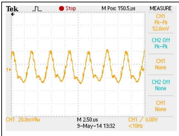
Figure 102: AEE01H36-L Ripple and Noise Measurement Vin = 48Vdc Load: Io = 1.67A Ch 1: Vo
