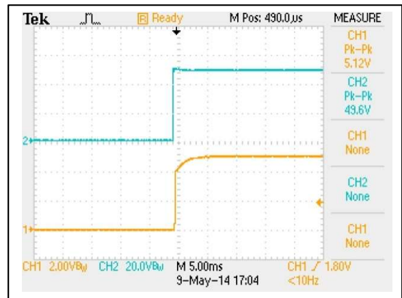
Figure 78: AEE08A36-L Output Voltage Startup Characteristic by Vin Vin = 48Vdc Load: Io = 8A Ch 1: Vo Ch 2: Vin
