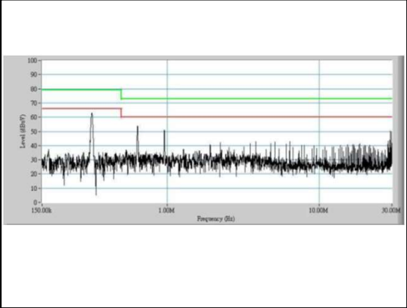
Figure 9: AEE08F18-L Conduction Emission of EN550122 Class A Vin = 24Vdc Load: Io = 8A
