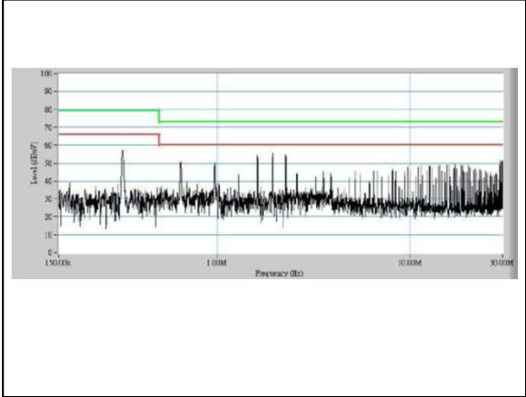
Figure 72: AEE08F36-L Conduction Emission of EN550122 Class A Vin = 48Vdc Load: Io = 8A
