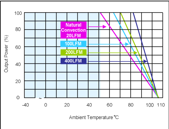
Figure 79: AEE08A36-L Derating Curves (without heatsink) Vin = 48Vdc Load: Io = 0 to 8A
