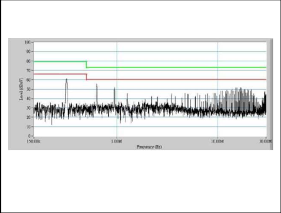
Figure 36: AEE02C18-L Conduction Emission of EN550122 Class A Vin = 24Vdc Load: Io = 2.67A
