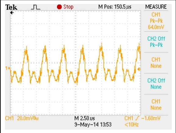
Figure 39: AEE01H18-L Ripple and Noise Measurement Vin = 24Vdc Load: Io = 1.67A Ch 1: Vo
