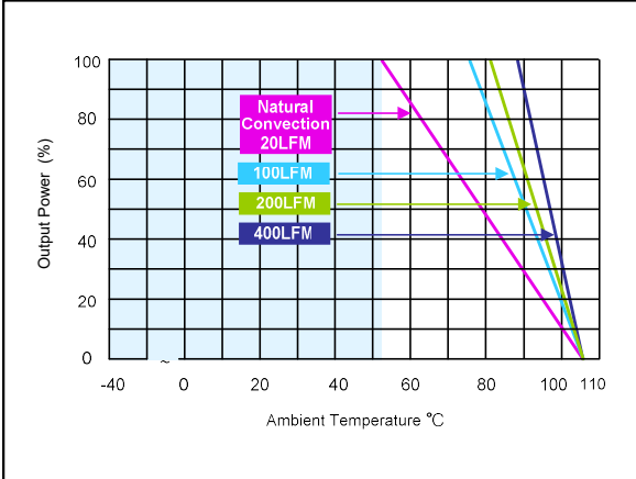
Figure 116: AEE01BB36-L Derating Curves (with heatsink) Vin = 48Vdc Load: Io = 0 to ±1.67A
