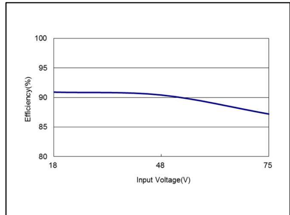
Figure 74: AEE08A36-L Efficiency Versus Input Voltage Curve Vin = 18 to 75Vdc Load: Io = 8A
