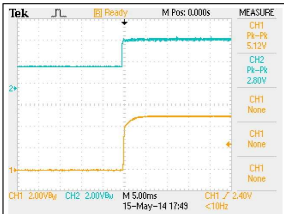
Figure 77: AEE08A36-L Output Voltage Startup Characteristic by On/Off Vin = 48Vdc Load: Io = 8A Ch 1: Vo Ch 2: Remote On/Off
