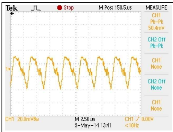
Figure 75: AEE08A36-L Ripple and Noise Measurement Vin = 48Vdc Load: Io = 8A Ch 1: Vo
