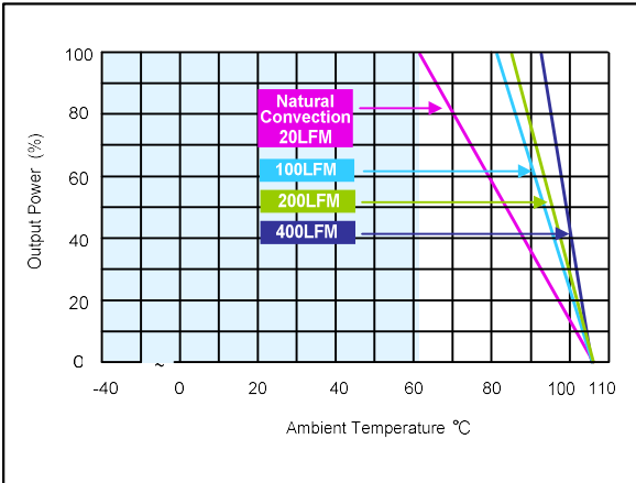
Figure 89: AEE03B36-L Derating Curves (with heatsink) Vin = 48Vdc Load: Io = 0 to 3.33A
