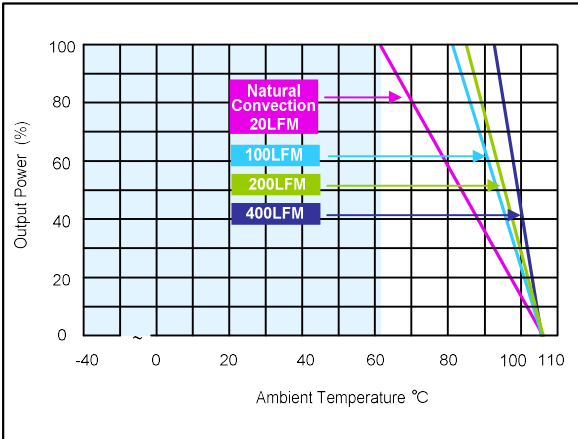
Figure 80: AEE08A36-L Derating Curves (with heatsink) Vin = 48Vdc Load: Io = 0 to 8A
