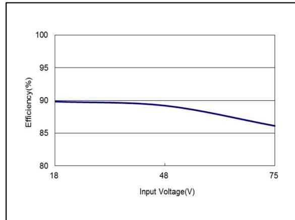
Figure 119: AEE01CC36-L Efficiency Versus Input Voltage Curve Vin = 18 to 75Vdc Load: Io = ±1.33A
