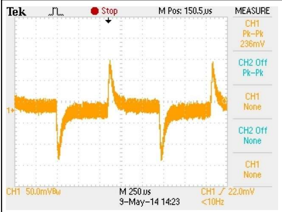
Figure 40: AEE01H18-L Transient Response Vin = 24Vdc Load: Io = 100% to 75% load change Ch 1: Vo
