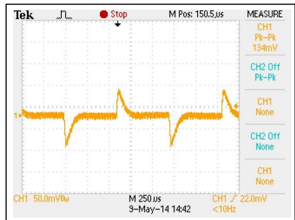
Figure 76: AEE08A36-L Transient Response Vin = 48Vdc Load: Io = 100% to 75% load change Ch 1: Vo
