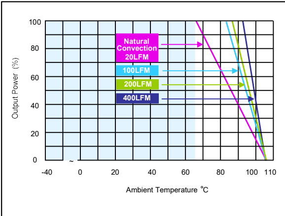
Figure 107: AEE01H36-L Derating Curves (with heatsink) Vin = 48Vdc Load: Io = 0 to 1.67A
