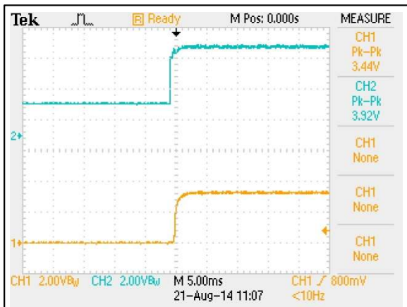
Figure 68: AEE08F36-L Output Voltage Startup Characteristic by On/Off Vin = 48Vdc Load: Io = 8A Ch 1: Vo Ch 2: Remote On/Off
