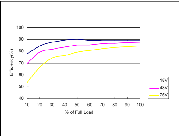
Figure 109: AEE01BB36-L Efficiency Versus Output Current Curve Vin = 18 to 75Vdc Load: Io = 0 to ±1.67A
