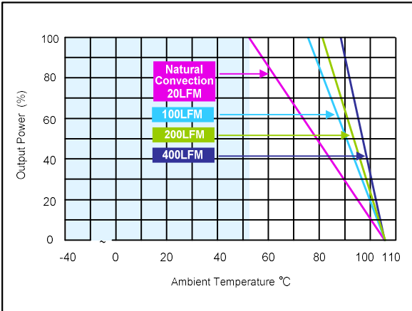
Figure 125: AEE01CC36-L Derating Curves (with heatsink) Vin = 48Vdc Load: Io = 0 to ±1.33A
