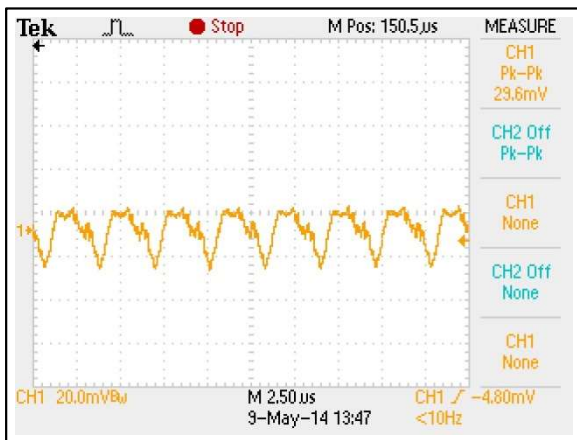
Figure 12: AEE08A18-L Ripple and Noise Measurement Vin = 24Vdc Load: Io = 8A Ch 1: Vo
