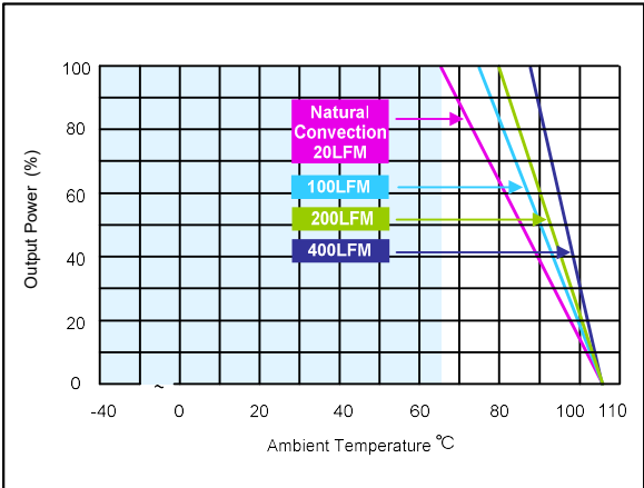
Figure 70: AEE08F36-L Derating Curves (without heatsink) Vin = 48Vdc Load: Io = 0 to 8A
