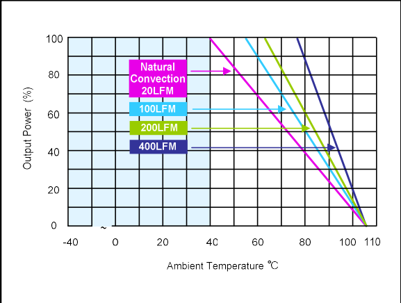
Figure 115: AEE01BB36-L Derating Curves (without heatsink) Vin = 48Vdc Load: Io = 0 to ±1.67A
