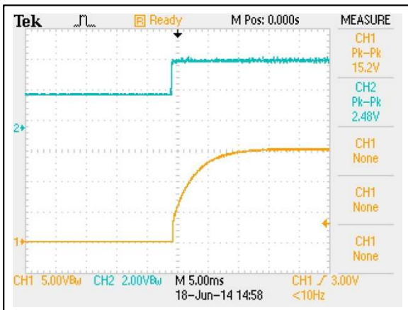
Figure 95: AEE02C36-L Output Voltage Startup Characteristic by On/Off Vin = 48Vdc Load: Io = 2.67A Ch 1: Vo Ch 2: Remote On/Off
