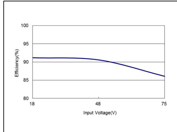
Figure 92: AEE02C36-L Efficiency Versus Input Voltage Curve Vin = 18 to 75Vdc Load: Io = 2.67A
