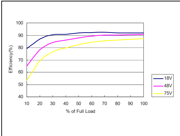
Figure 82: AEE03B36-L Efficiency Versus Output Current Curve Vin = 18 to 75Vdc Load: Io = 0 to 3.33A
