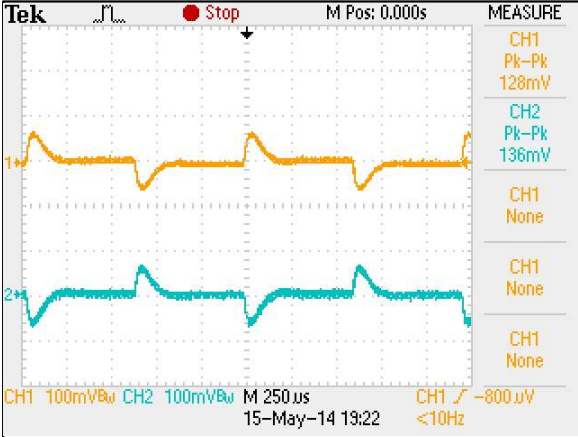
Figure 112: AEE01BB36-L Transient Response Vin = 48Vdc Load: Io = 100% to 75% load change Ch 1: Vo1 Ch 2: Vo2
