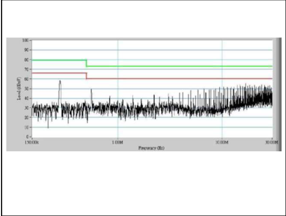
Figure 45: AEE01H18-L Conduction Emission of EN550122 Class A Vin = 24Vdc Load: Io = 1.67A
