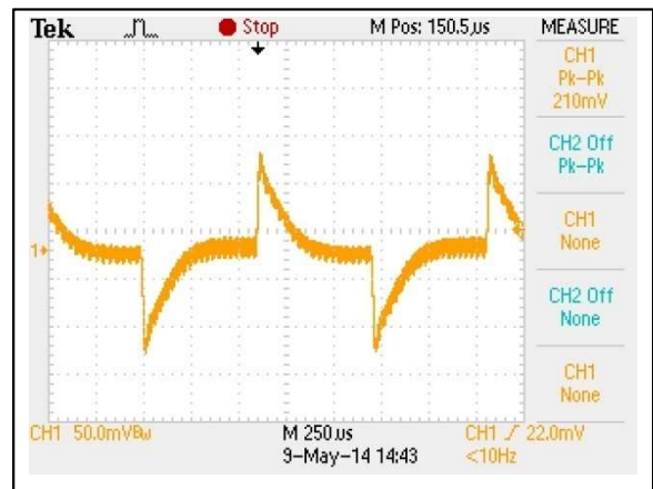
Figure 67: AEE08F36-L Transient Response Vin = 48Vdc Load: Io = 100% to 75% load change Ch 1: Vo
