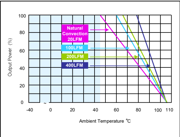
Figure 34: AEE02C18-L Derating Curves (without heatsink) Vin = 24Vdc Load: Io = 0 to 2.67A
