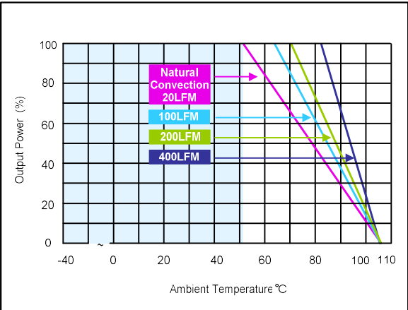
Figure 97: AEE02C36-L Derating Curves (without heatsink) Vin = 48Vdc Load: Io = 0 to 2.67A
