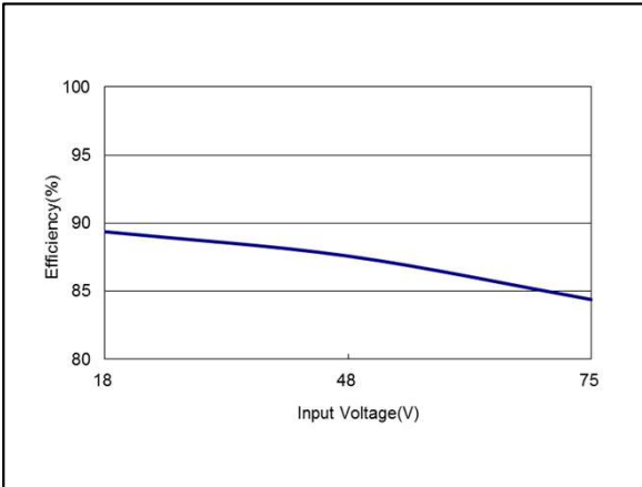
Figure 110: AEE01BB36-L Efficiency Versus Input Voltage Curve Vin = 18 to 75Vdc Load: Io = ±1.67A
