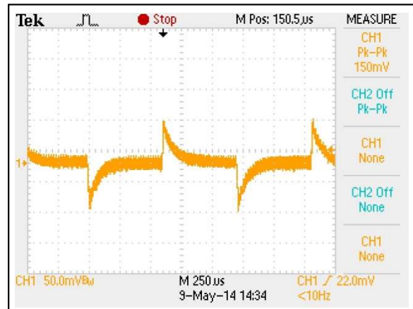
Figure 85: AEE03B36-L Transient Response Vin = 48Vdc Load: Io = 100% to 75% load change Ch 1: Vo
