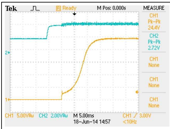
Figure 104: AEE01H36-L Output Voltage Startup Characteristic by On/Off Vin = 48Vdc Load: Io = 1.67A Ch 1: Vo Ch 2: Remote On/Off
