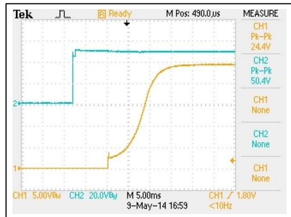
Figure 105: AEE01H36-L Output Voltage Startup Characteristic by Vin Vin = 48Vdc Load: Io = 1.67A Ch 1: Vo Ch 2: Vin
