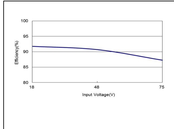
Figure 83: AEE03B36-L Efficiency Versus Input Voltage Curve Vin = 18 to 75Vdc Load: Io = 3.33A
