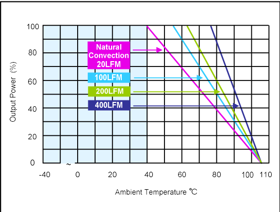
Figure 124: AEE01CC36-L Derating Curves (without heatsink) Vin = 48Vdc Load: Io = 0 to ±1.33A
