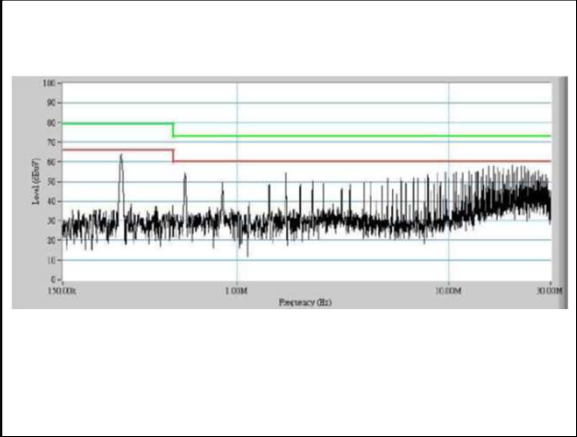
Figure 108: AEE01H36-L Conduction Emission of EN550122 Class A Vin = 48Vdc Load: Io = 1.67A
