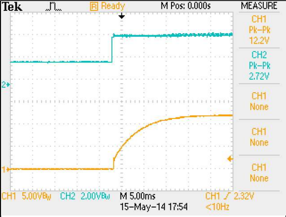
Figure 113: AEE01BB36-L Output Voltage Startup Characteristic by On/Off Vin = 48Vdc Load: Io = ±1.67A Ch 1: Vo Ch 2: Remote On/Off
