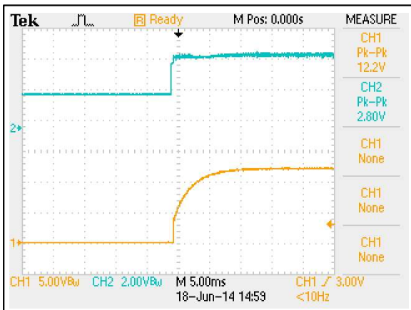
Figure 86: AEE03B36-L Output Voltage Startup Characteristic by On/Off Vin = 48Vdc Load: Io = 3.33A Ch 1: Vo Ch 2: Remote On/Off
