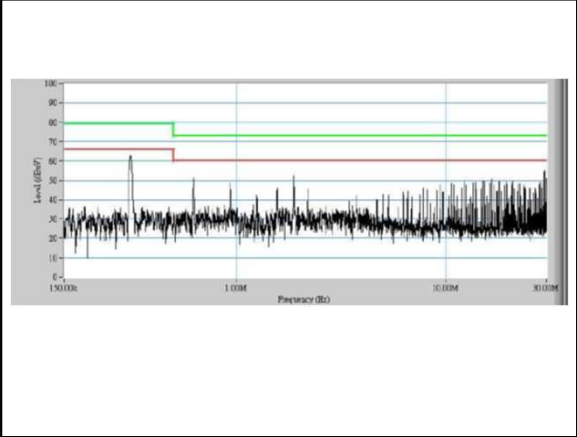
Figure 81: AEE08A36-L Conduction Emission of EN550122 Class A Vin = 48Vdc Load: Io = 8A
