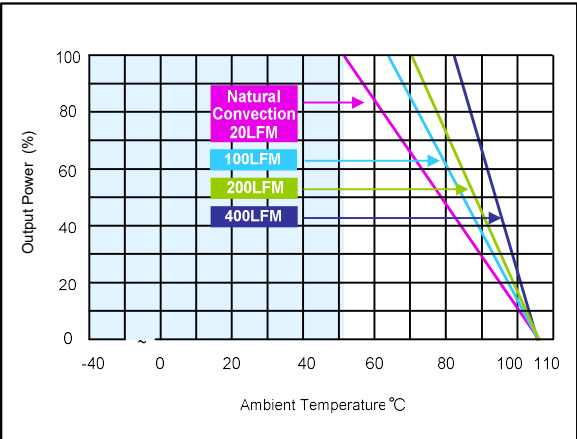
Figure 16: AEE08A18-L Derating Curves (without heatsink) Vin = 24Vdc Load: Io = 0 to 8A
