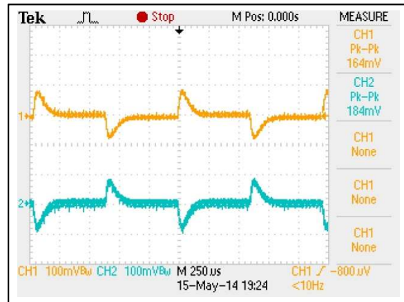
Figure 58: AEE01CC18-L Transient Response Vin = 48Vdc Load: Io = 100% to 75% load change Ch 1: Vo1 Ch 1: Vo2
