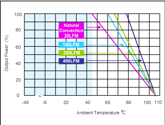
Figure 25: AEE03B18-L Derating Curves (without heatsink) Vin = 24Vdc Load: Io = 0 to 3.33A
