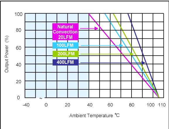
Figure 61: AEE01CC18-L Derating Curves (without heatsink) Vin = 48Vdc Load: Io = 0 to ±1.33A
