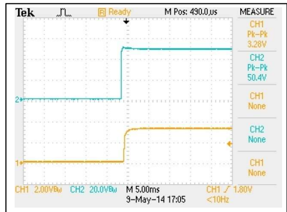
Figure 69: AEE08F36-L Output Voltage Startup Characteristic by Vin Vin = 48Vdc Load: Io = 8A Ch 1: Vo Ch 2: Vin
