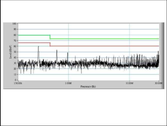
Figure 63: AEE01CC18-L Conduction Emission of EN550122 Class A Vin = 48Vdc Load: Io = ±1.33A
