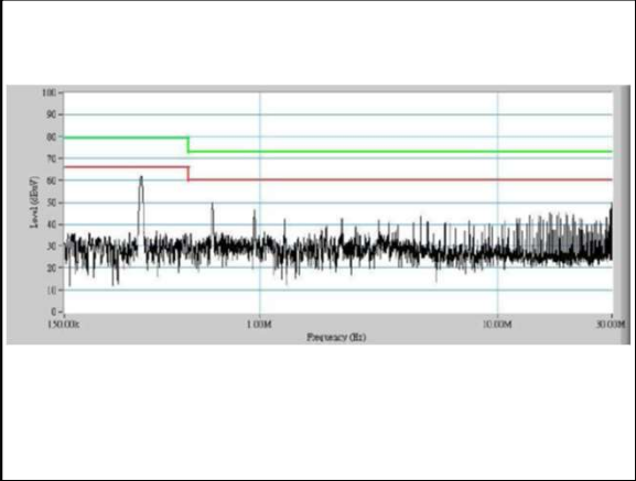
Figure 18: AEE08A18-L Conduction Emission of EN550122 Class A Vin = 24Vdc Load: Io = 8A
