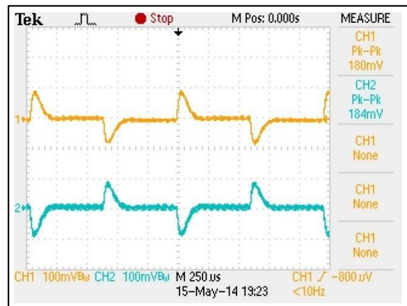
Figure 121: AEE01CC36-L Transient Response Vin = 48Vdc Load: Io = 100% to 75% load change Ch 1: Vo1 Ch 2: Vo2
