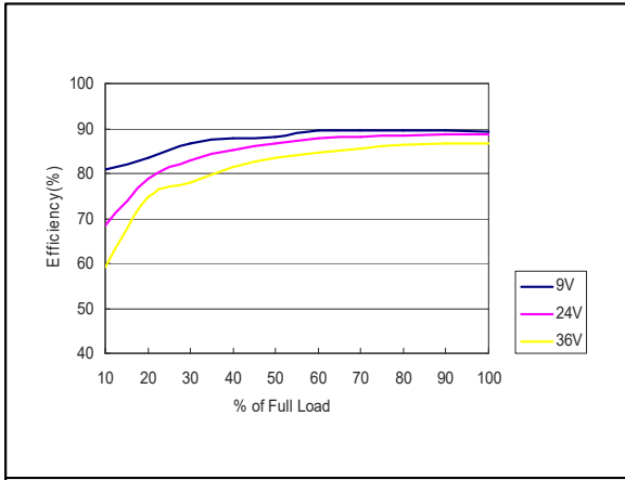
Figure 46: AEE01BB18-L Efficiency Versus Output Current Curve Vin = 9 to 36Vdc Load: Io = 0 to ±1.67A
