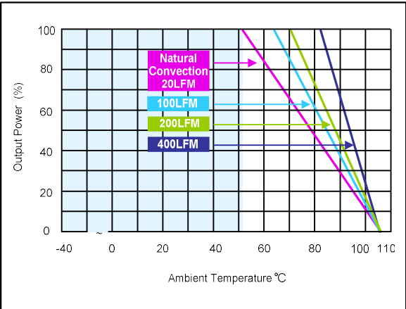
Figure 88: AEE03B36-L Derating Curves (without heatsink) Vin = 48Vdc Load: Io = 0 to 3.33A
