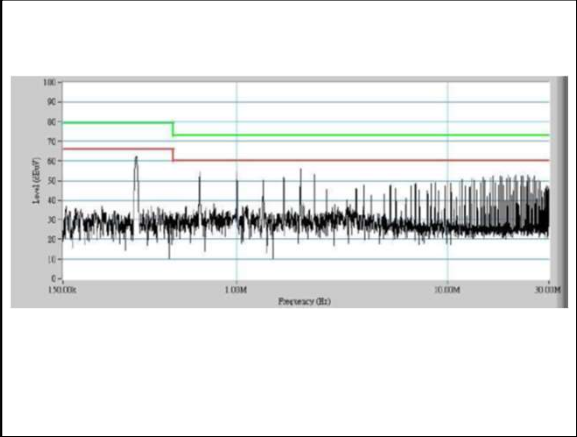
Figure 99: AEE02C36-L Conduction Emission of EN550122 Class A Vin = 48Vdc Load: Io = 2.67A
