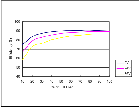
Figure 55: AEE01CC18-L Efficiency Versus Output Current Curve Vin = 18 to 75Vdc Load: Io = 0 to ±1.33A
