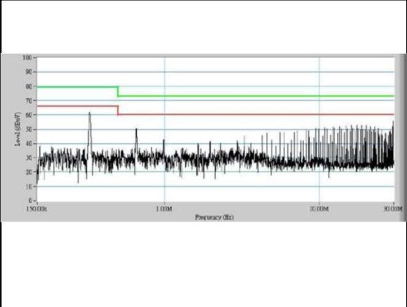
Figure 126: AEE01CC36-L Conduction Emission of EN550122 Class A Vin = 48Vdc Load: Io = ±1.33A
