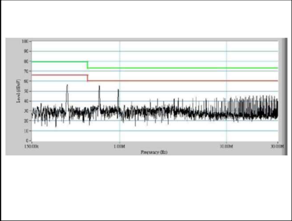
Figure 54: AEE01BB18-L Conduction Emission of EN550122 Class A Vin = 24Vdc Load: Io = ±1.67A
