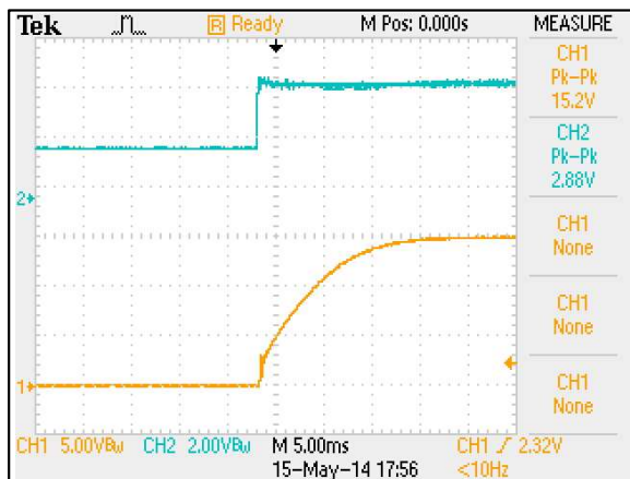
Figure 122: AEE01CC36-L Output Voltage Startup Characteristic by On/Off Vin = 48Vdc Load: Io = ±1.33A Ch 1: Vo Ch 2: Remote On/Off
