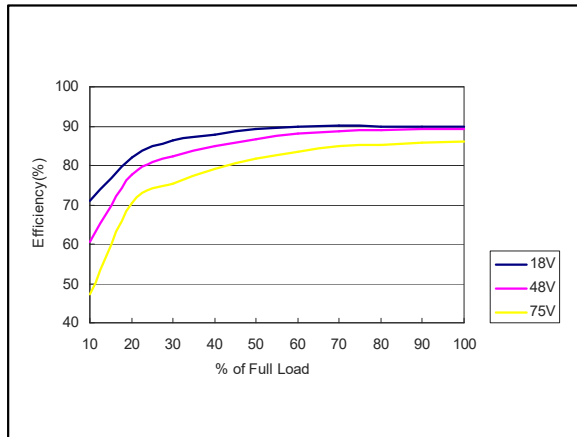
Figure 118: AEE01CC36-L Efficiency Versus Output Current Curve Vin = 18 to 75Vdc Load: Io = 0 to ±1.33A
