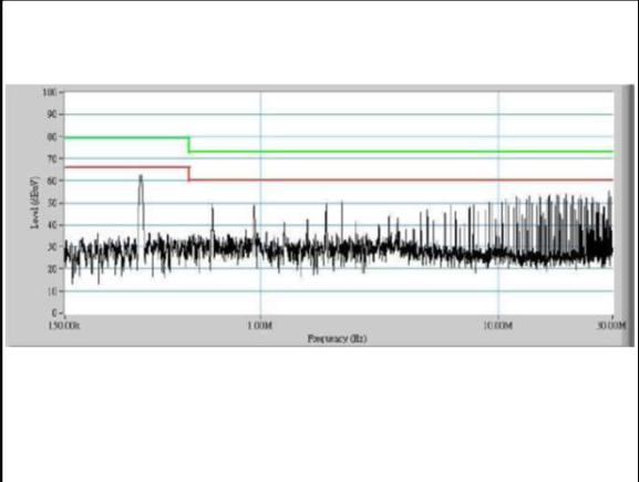
Figure 117: AEE01BB36-L Conduction Emission of EN550122 Class A Vin = 48Vdc Load: Io = ±1.67A
