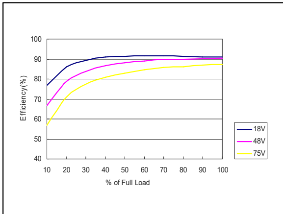
Figure 73: AEE08A36-L Efficiency Versus Output Current Curve Vin = 18 to 75Vdc Load: Io = 0 to 8A
