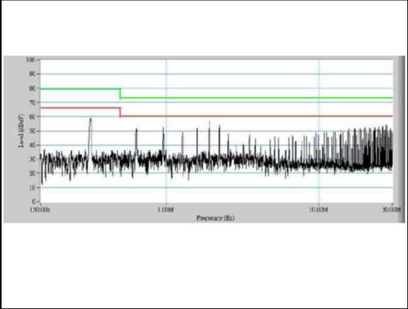
Figure 90: AEE03B36-L Conduction Emission of EN550122 Class A Vin = 48Vdc Load: Io = 3.33A
