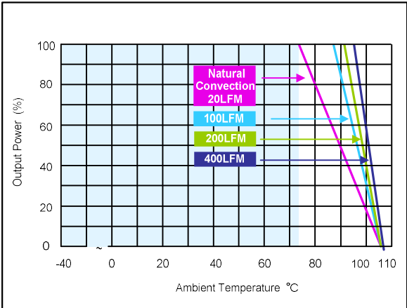
Figure 71: AEE08F36-L Derating Curves (with heatsink) Vin = 48Vdc Load: Io = 0 to 8A
