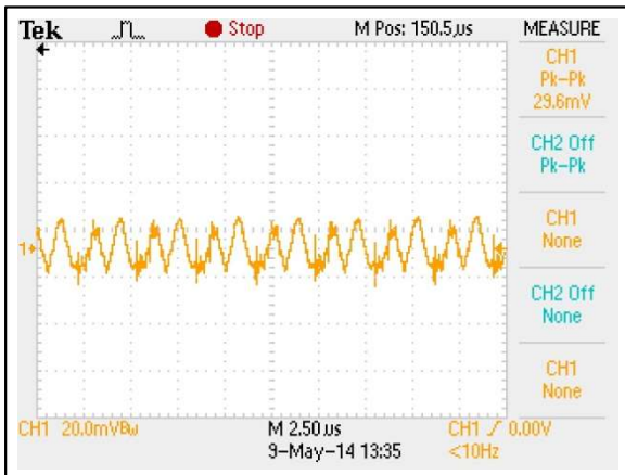
Figure 84: AEE03B36-L Ripple and Noise Measurement Vin = 48Vdc Load: Io = 3.33A Ch 1: Vo
