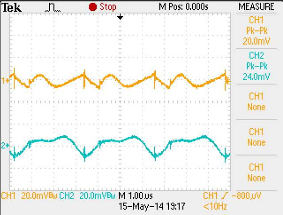
Figure 111: AEE01BB36-L Ripple and Noise Measurement Vin = 48Vdc Load: Io = ±1.67A Ch 1: Vo1 Ch 2: Vo2
