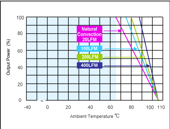
Figure 7: AEE08F18-L Derating Curves (without heatsink) Vin = 24Vdc Load: Io = 0 to 8A
