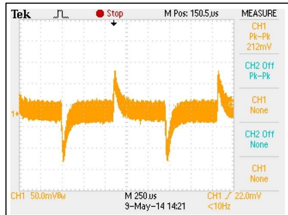
Figure 103: AEE01H36-L Transient Response Vin = 48Vdc Load: Io = 100% to 75% load change Ch 1: Vo
