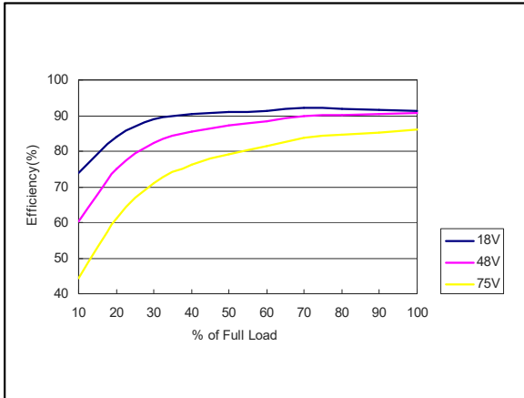
Figure 91: AEE02C36-L Efficiency Versus Output Current Curve Vin = 18 to 75Vdc Load: Io = 0 to 2.67A
