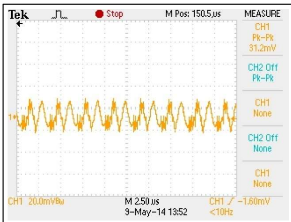
Figure 30: AEE02C18-L Ripple and Noise Measurement Vin = 24Vdc Load: Io = 2.67A Ch 1: Vo
