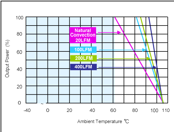
Figure 98: AEE02C36-L Derating Curves (with heatsink) Vin = 48Vdc Load: Io = 0 to 2.67A
