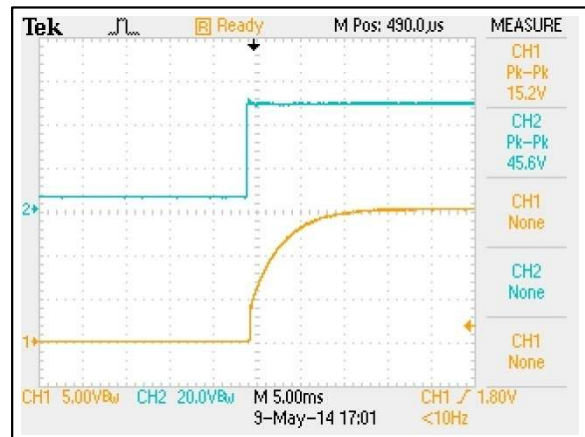
Figure 96: AEE02C36-L Output Voltage Startup Characteristic by Vin Vin = 48Vdc Load: Io = 2.67A Ch 1: Vo Ch 2: Vin
