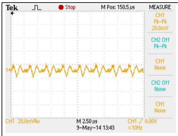
Figure 66: AEE08F36-L Ripple and Noise Measurement Vin = 48Vdc Load: Io = 8A Ch 1: Vo
