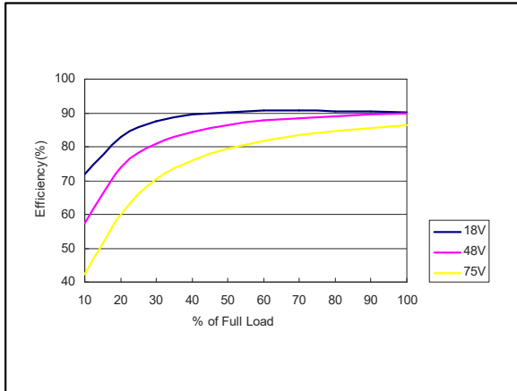
Figure 64: AEE08F36-L Efficiency Versus Output Current Curve Vin = 18 to 75Vdc Load: Io = 0 to 8A
