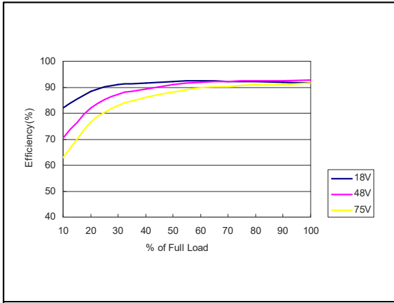
Figure 100: AEE01H36-L Efficiency Versus Output Current Curve Vin = 18 to 75Vdc Load: Io = 0 to 1.67A
