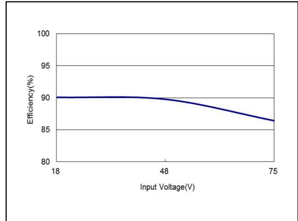
Figure 65: AEE08F36-L Efficiency Versus Input Voltage Curve Vin = 18 to 75Vdc Load: Io = 8A
