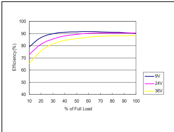
Figure 10: AEE08A18-L Efficiency Versus Output Current Curve Vin = 9 to 36Vdc Load: Io = 0 to 8A
