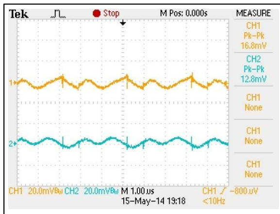
Figure 120: AEE01CC36-L Ripple and Noise Measurement Vin = 48Vdc Load: Io = ±1.33A Ch 1: Vo1 Ch 2: Vo2
