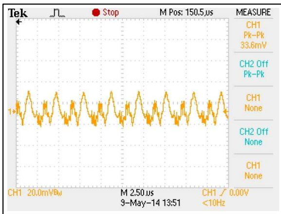
Figure 21: AEE03B18-L Ripple and Noise Measurement Vin = 24Vdc Load: Io = 3.33A Ch 1: Vo
