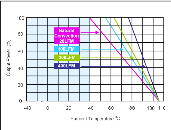
Figure 52: AEE01BB18-L Derating Curves (without heatsink) Vin = 24Vdc Load: Io = 0 to ±1.67A
