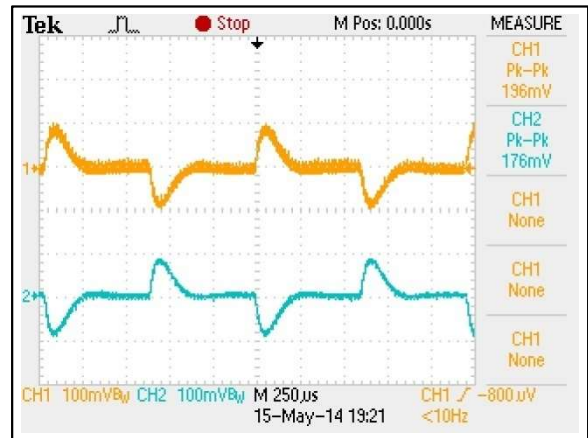
Figure 49: AEE01BB18-L Transient Response Vin = 24Vdc Load: Io = 100% to 75% load change Ch 1: Vo1 Ch 1: Vo2
