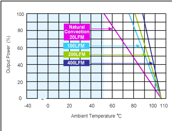
Figure 62: AEE01CC18-L Derating Curves (with heatsink) Vin = 48Vdc Load: Io = 0 to ±1.33A
