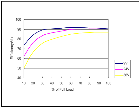
Figure 28: AEE02C18-L Efficiency Versus Output Current Curve Vin = 9 to 36Vdc Load: Io = 0 to 2.67A
