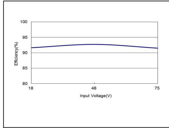
Figure 101: AEE01H36-L Efficiency Versus Input Voltage Curve Vin = 18 to 75Vdc Load: Io = 1.67A
