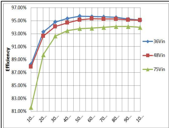
Figure 9: ADO300-48S12 Efficiency vs. output current, Ta=25oC, Vo=11.9V Loading: Io = 10% increment to 26A
