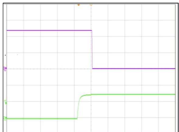
Figure 6: ADO300-48S12 Remote OFF Waveform (200mS/div)
