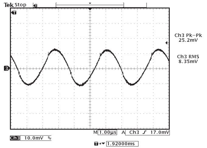
Figure 8: Typical Ripple and Noise* (Channel 3: Vo)
