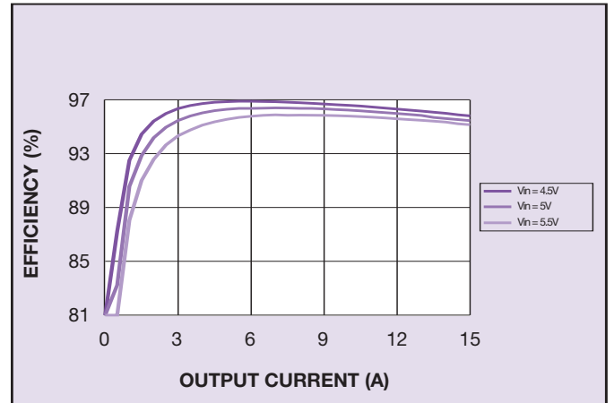
Figure 18: Efficiency vs Load
