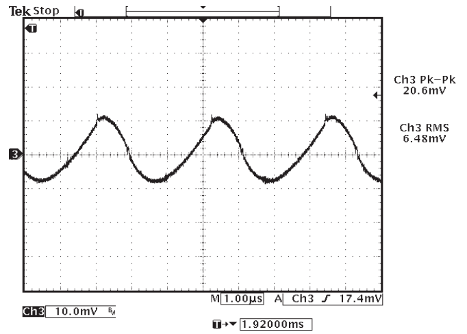
Figure 16: Typical Ripple and Noise* (Channel 3: Vo)
