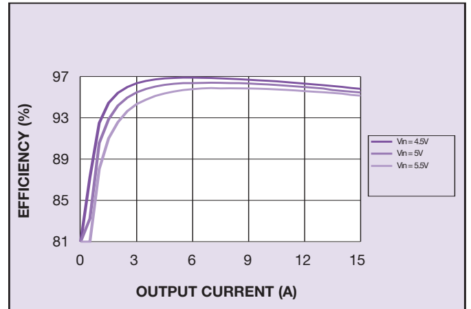
Figure 10: Efficiency vs Load
