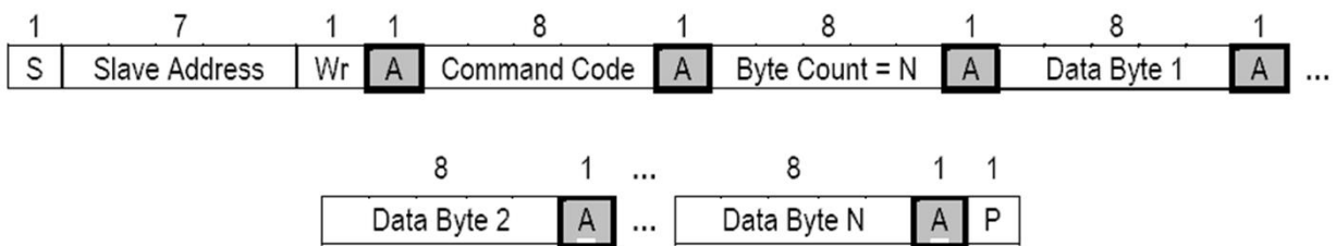
Figure 5-17: Block Write
