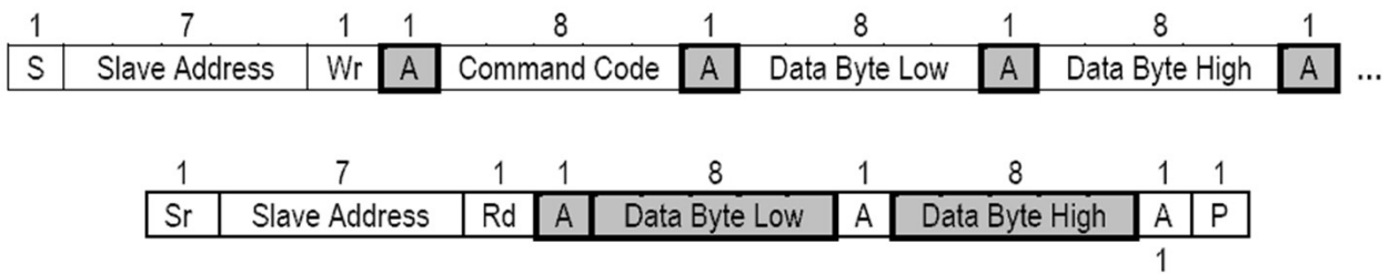
Figure 5-15: Process Call
