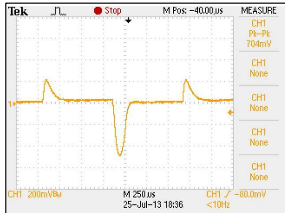
Figure 31: ERM03H72 Transient Response Vin = 72Vdc Load: Io = 100% to 75% load change Ch 1: Vo
