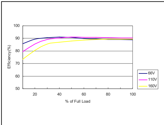
Figure 37: ERM15A110 Efficiency Versus Output Current Curve Vin = 66 to 160Vdc Load: Io = 0 to 15A
