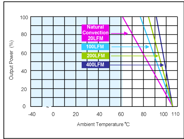
Figure 17: ERM06B72 Derating Curve with Heatsink Vin = 72Vdc Load: Io = 0 to 6.25A
