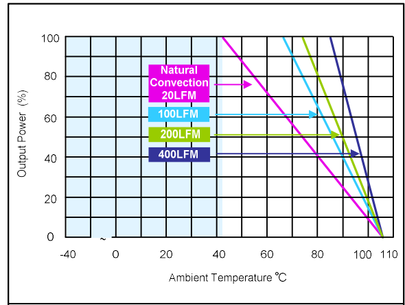
Figure 44: ERM15A110 Derating Curve with Heatsink Vin = 110Vdc Load: Io = 0 to 15A
