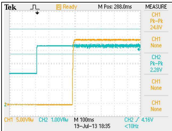
Figure 68: ERM03H110 Output Voltage Startup Characteristic by On/Off Vin = 110Vdc Load: Io = 3.125A Ch 1: Vo Ch 2: Remote On/Off
