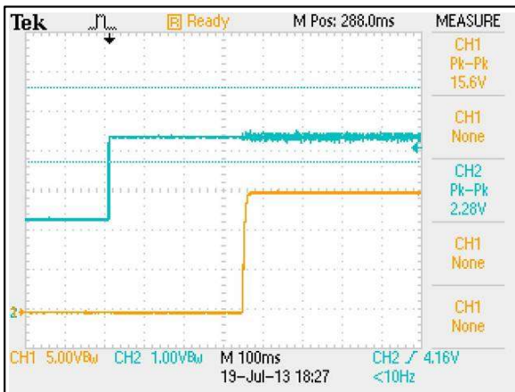
Figure 59: ERM05C110 Output Voltage Startup Characteristic by On/Off Vin = 110Vdc Load: Io = 5A Ch 1: Vo Ch 2: Remote On/Off
