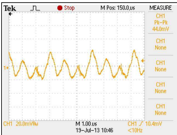
Figure 66: ERM03H110 Typical Output Ripple and Noise. Vin = 110Vdc Load: Io = 3.125A Ch 1: Vo
