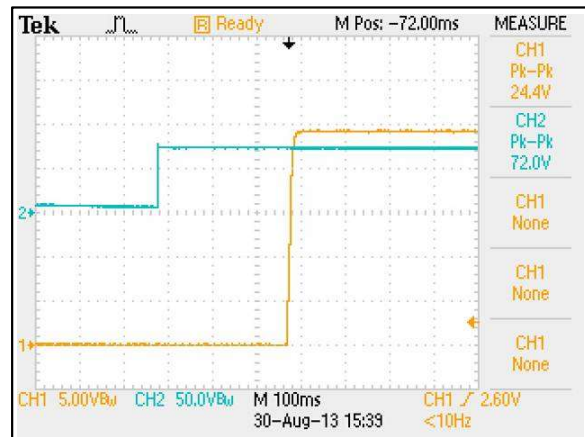
Figure 33: ERM03H72 Output Voltage Startup Characteristic by Vin Vin = 72Vdc Load: Io = 3.125A Ch 1: Vo Ch 2: Vin
