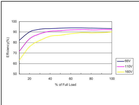
Figure 55: ERM05C110 Efficiency Versus Output Current Curve Vin = 66 to 160Vdc Load: Io = 0 to 5A
