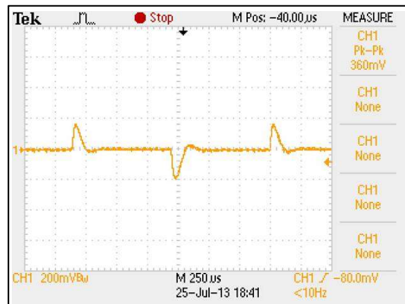
Figure 49: ERM06B110 Transient Response Vin = 110Vdc Load: Io = 100% to 75% load change Ch 1: Vo
