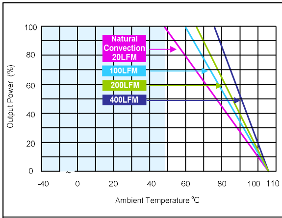
Figure 52: ERM06B110 Derating Curve without Heatsink Vin = 110Vdc Load: Io = 0 to 6.25A
