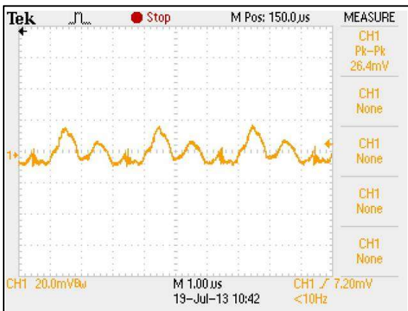
Figure 57: ERM05C110 Typical Output Ripple and Noise. Vin = 110Vdc Load: Io = 5A Ch 1: Vo
