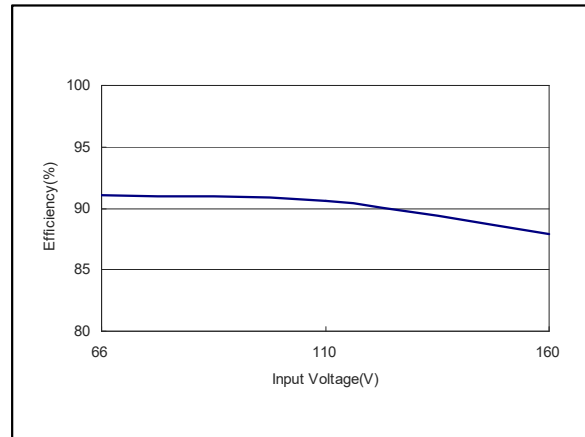
Figure 65: ERM03H110 Efficiency Versus Input Voltage Curve Vin = 66 to 160Vdc Load: Io = 0 to 3.125A
