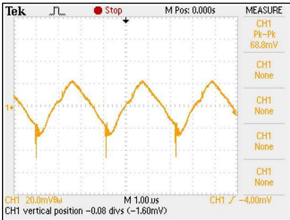
Figure 3: ERM15A72 Typical Output Ripple and Noise. Vin = 72Vdc Load: Io = 15A Ch 1: Vo
