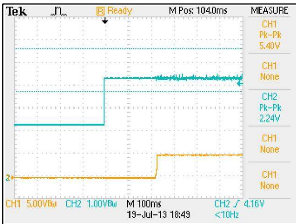
Figure 5: ERM15A72 Output Voltage Startup Characteristic by On/Off Vin = 72Vdc Load: Io = 15A Ch 1: Vo Ch 2: Remote On/Off
