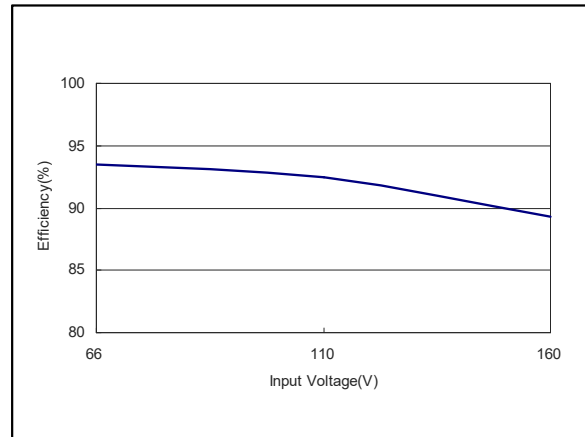
Figure 47: ERM06B110 Efficiency Versus Input Voltage Curve Vin = 66 to 160Vdc Load: Io = 0 to 6.25A
