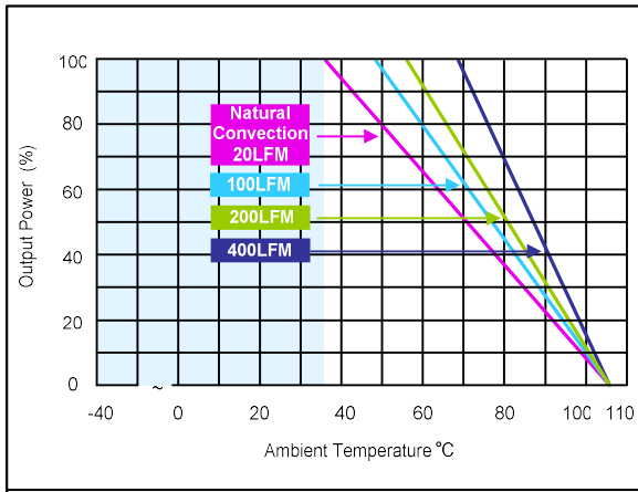
Figure 43: ERM15A110 Derating Curve without Heatsink Vin = 110Vdc Load: Io = 0 to 15A
