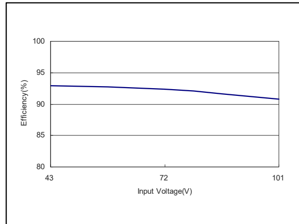
Figure 20: ERM05C72 Efficiency Versus Input Voltage Curve Vin = 43 to 101Vdc Load: Io = 0 to 5A
