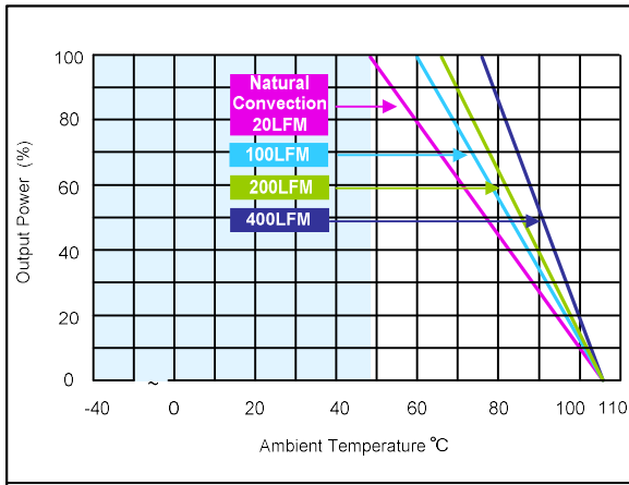
Figure 61: ERM05C110 Derating Curve without Heatsink Vin = 110Vdc Load: Io = 0 to 5A
