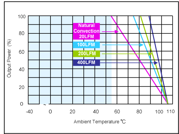
Figure 53: ERM06B110 Derating Curve with Heatsink Vin = 110Vdc Load: Io = 0 to 6.25A
