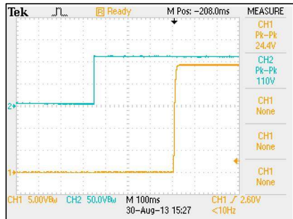
Figure 69: ERM03H110 Output Voltage Startup Characteristic by Vin Vin = 110Vdc Load: Io = 3.125A Ch 1: Vo Ch 2: Vin
