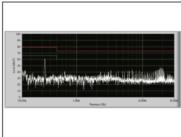
Figure 18: ERM06B72 Conduction Emission of EN55011 Class A Vin = 72Vdc Load: Io = 6.25A
