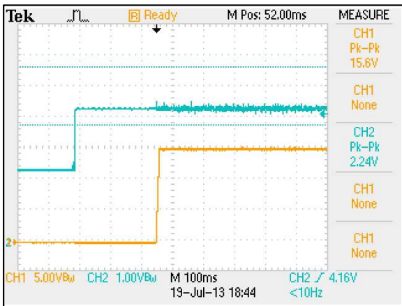
Figure 23: ERM05C72 Output Voltage Startup Characteristic by On/Off Vin = 72Vdc Load: Io = 5A Ch 1: Vo Ch 2: Remote On/Off
