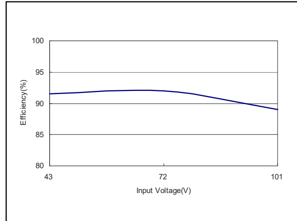
Figure 29: ERM03H72 Efficiency Versus Input Voltage Curve Vin = 43 to 101Vdc Load: Io = 0 to 3.125A
