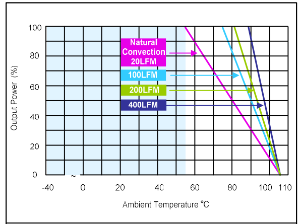
Figure 35: ERM03H72 Derating Curve with Heatsink Vin = 72Vdc Load: Io = 0 to 3.125A
