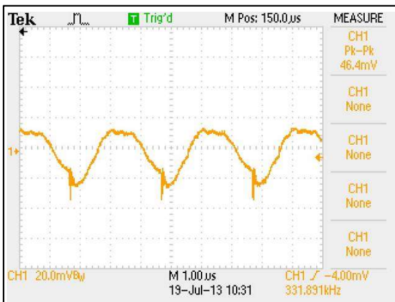
Figure 39: ERM15A110 Typical Output Ripple and Noise. Vin = 110Vdc Load: Io = 15A Ch 1: Vo
