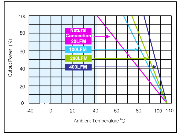
Figure 8: ERM15A72 Derating Curve with Heatsink Vin = 72Vdc Load: Io = 0 to 15A
