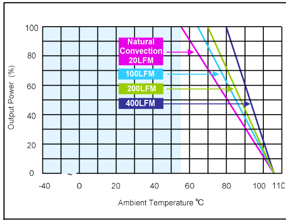
Figure 16: ERM06B72 Derating Curve without Heatsink Vin = 72Vdc Load: Io = 0 to 6.25A
