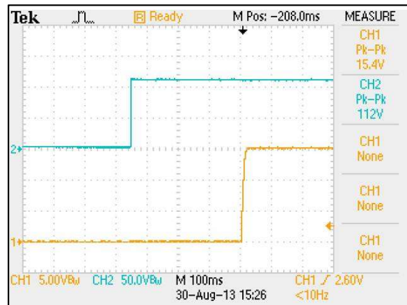
Figure 60: ERM05C110 Output Voltage Startup Characteristic by Vin Vin = 110Vdc Load: Io = 5A Ch 1: Vo Ch 2: Vin
