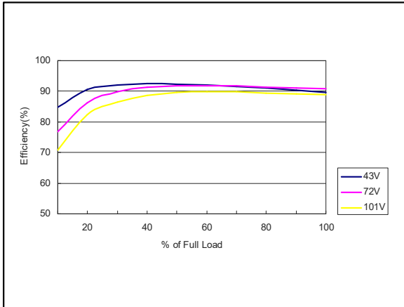
Figure 1: ERM15A72 Efficiency Versus Output Current Curve Vin = 43 to 101Vdc Load: Io = 0 to 15A
