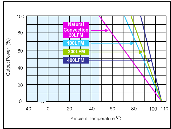
Figure 71: ERM03H110 Derating Curve with Heatsink Vin = 110Vdc Load: Io = 0 to 3.125A
