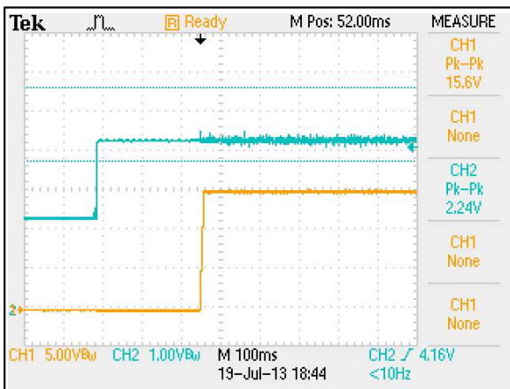
Figure 21: ERM05C72 Typical Output Ripple and Noise. Vin = 72Vdc Load: Io = 5A Ch 1: Vo
