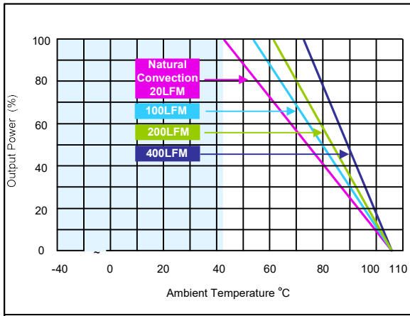
Figure 70: ERM03H110 Derating Curve without Heatsink Vin = 110Vdc Load: Io = 0 to 3.125A
