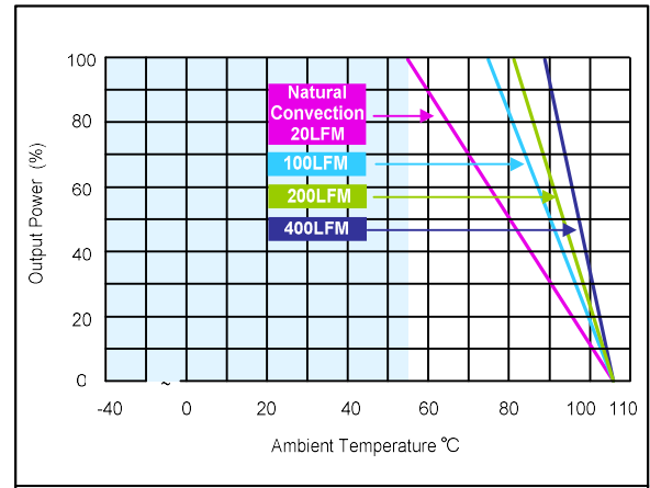
Figure 62: ERM05C110 Derating Curve with Heatsink Vin = 110Vdc Load: Io = 0 to 5A
