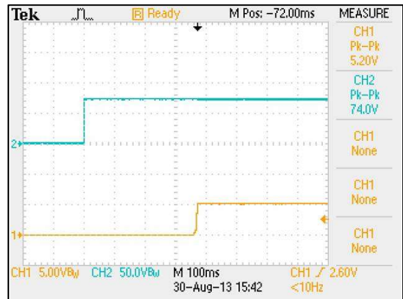
Figure 6: ERM15A72 Output Voltage Startup Characteristic by Vin Vin = 72Vdc Load: Io = 15A Ch 1: Vo Ch 2: Vin
