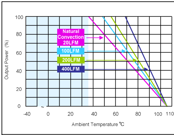
Figure 7: ERM15A72 Derating Curve without Heatsink Vin = 72Vdc Load: Io = 0 to 15A
