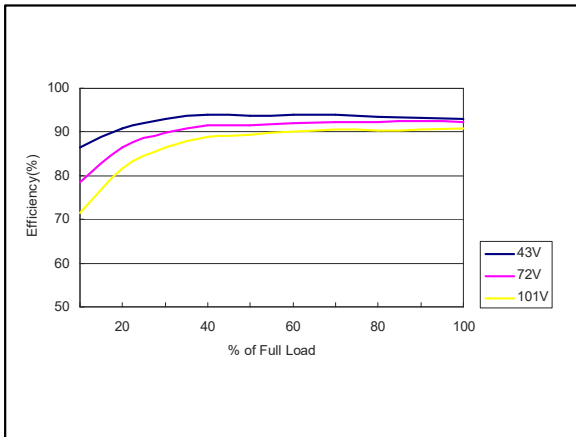
Figure 19: ERM05C72 Efficiency Versus Output Current Curve Vin = 43 to 101Vdc Load: Io = 0 to 5A
