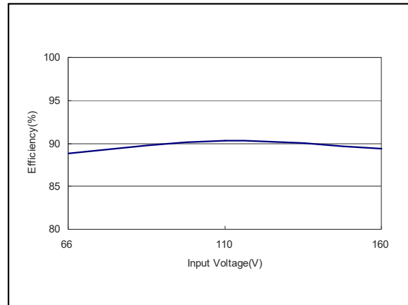
Figure 38: ERM15A110 Efficiency Versus Input Voltage Curve Vin = 66 to 160Vdc Load: Io = 0 to 15A
