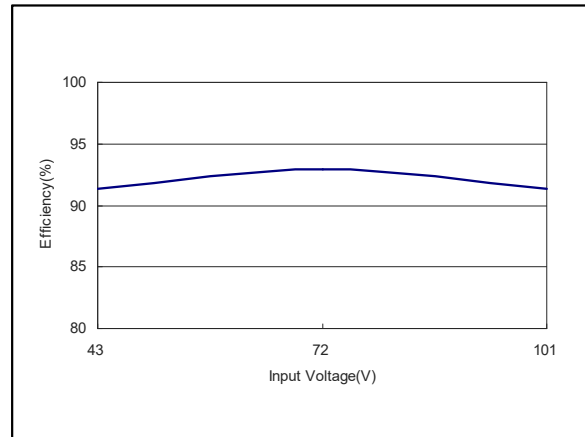
Figure 11: ERM06B72 Efficiency Versus Input Voltage Curve Vin = 43 to 101Vdc Load: Io = 0 to 6.25A
