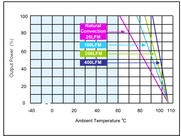
Figure 26: ERM05C72 Derating Curve with Heatsink Vin = 72Vdc Load: Io = 0 to 5A
