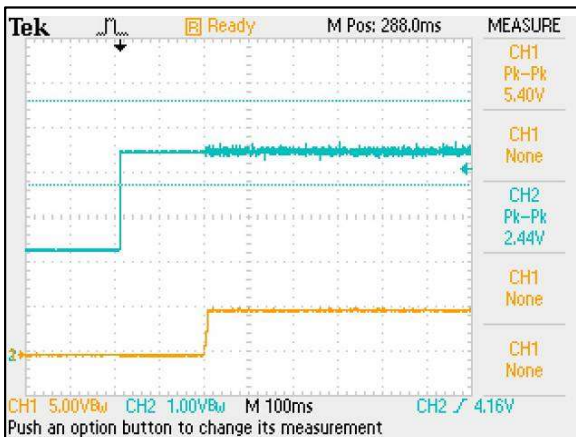
Figure 41: ERM15A110 Output Voltage Startup Characteristic by On/Off Vin = 110Vdc Load: Io = 15A Ch 1: Vo Ch 2: Remote On/Off
