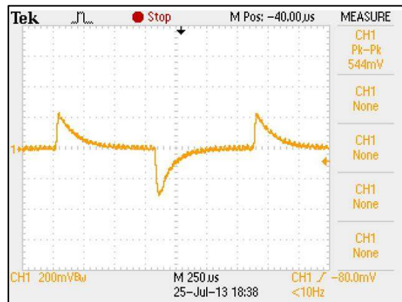
Figure 67: ERM03H110 Transient Response Vin = 110Vdc Load: Io = 100% to 75% load change Ch 1: Vo
