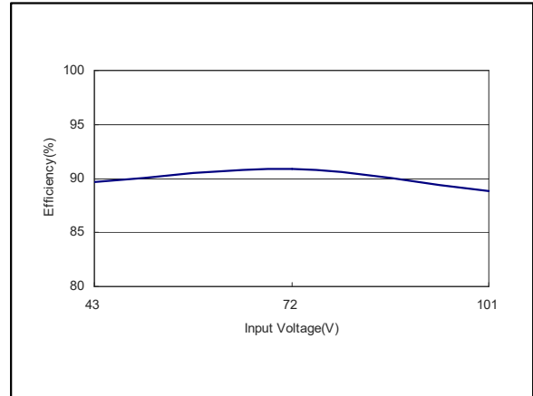
Figure 2: ERM15A72 Efficiency Versus Input Voltage Curve Vin = 43 to 101Vdc Load: Io = 0 to 15A
