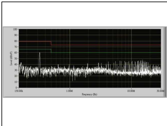
Figure 72: ERM03H110 Conduction Emission of EN55011 Class A Vin = 110Vdc Load: Io = 3.125A
