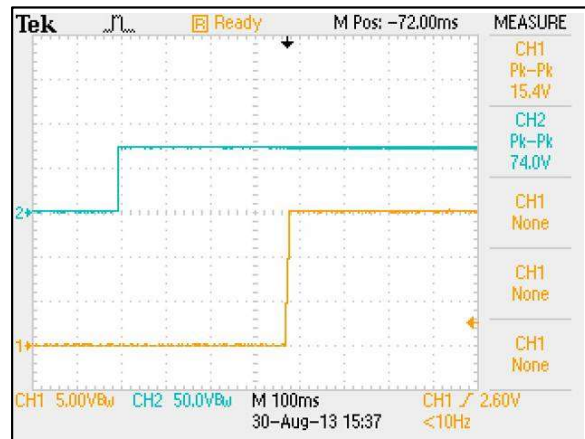
Figure 24: ERM05C72 Output Voltage Startup Characteristic by Vin Vin = 72Vdc Load: Io = 5A Ch 1: Vo Ch 2: Vin
