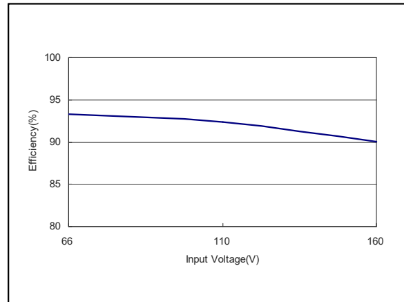
Figure 56: ERM05C110 Efficiency Versus Input Voltage Curve Vin = 66 to 160Vdc Load: Io = 0 to 5A
