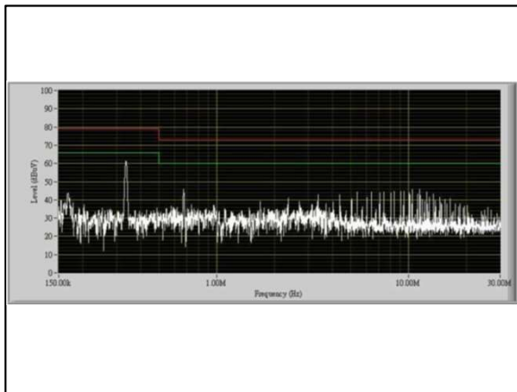
Figure 36: ERM03H72 Conduction Emission of EN55011 Class A Vin = 72Vdc Load: Io = 3.125A
