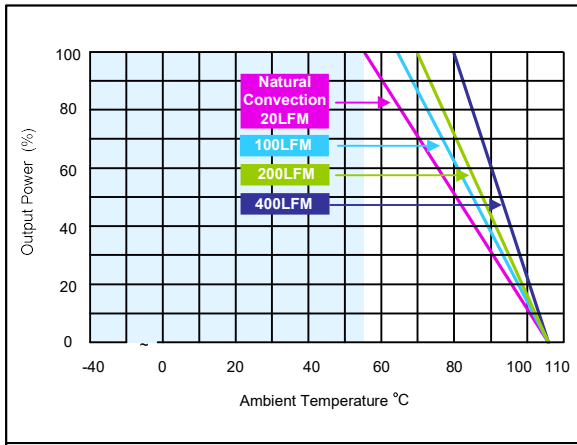
Figure 25: ERM05C72 Derating Curve without Heatsink Vin = 72Vdc Load: Io = 0 to 5A
