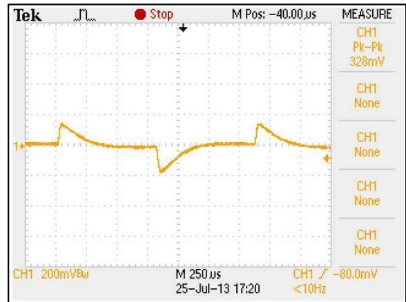
Figure 4: ERM15A72 Transient Response Vin = 72Vdc Load: Io = 100% to 75% load change Ch 1: Vo
