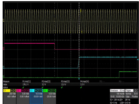
Figure 4: DS2400SPE-3 Turn-on Delay via PSOn Vin = 180Vac Load: I_o = 196.7A I_{SB} = 3.5A Ch 1: AC Mains Ch 2: V_{SB} Ch 3: V_o Ch 4: PWOK
