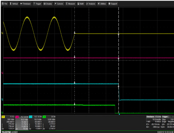
Figure 5: DS2400SPE-3 Hold-up Time Vin = 90Vac Load: I_o = 114.75A I_{SB} = 3.5A Ch 1: AC Mains Ch 2: V_{SB} Ch 3: V_o Ch 4: PWOK
