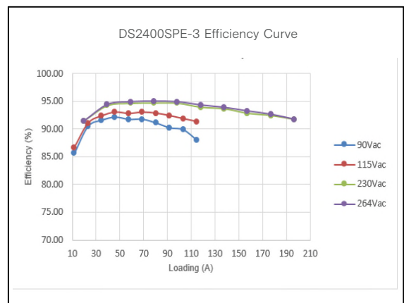
Figure 12: DS2400SPE-3 Efficiency Curve @ 25°C Loading: I_{o,max} increment to 114.75A (90/115Vac) and 196.7A (230/264Vac), I_{o,min} = 10\%I_{o,max} increment to 3.5A
