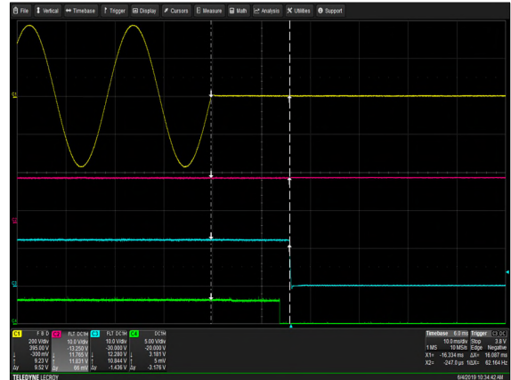
Figure 6: DS2400SPE-3 Hold-up Time Vin = 264Vac Load: I_o = 196.7A I_{SB} = 3.5A Ch 1: AC Mains Ch 2: V_{SB} Ch 3: V_o Ch 4: PWOK
