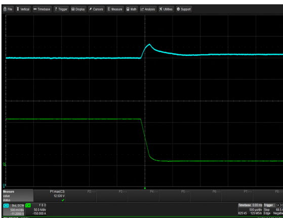
Figure 11: DS2400SPE-3 Transient Response - V_o Deviation 100% to 40% load change 0.5A/ \mu s slew rate V_{in} = 230V_{ac} Ch 3: V_o Ch 4: I_o
