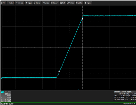
Figure 7: DS2400SPE-3 Output Voltage Startup Characteristic V_{in} = 90V_{ac} Load: I_o = 114.8A I_{SB} = 3.5A Ch 3: V_o
