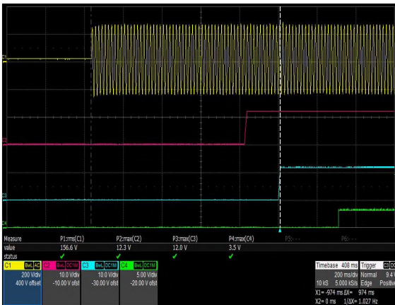
Figure 3: DS2400SPE-3 Turn-on Delay via AC Mains Vin = 180Vac Load: I_o = 196.7A I_{SB} = 3.5A Ch 1: AC Mains Ch 2: V_{SB} Ch 3: V_o Ch 4: PWOK
