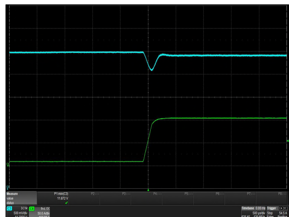
Figure 10: DS2400SPE-3 Transient Response - V_o Deviation 40% to 100% load change 0.5A/ \mu s slew rate V_{in} = 230V_{ac} Ch 3: V_o Ch 4: I_o
