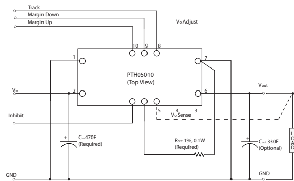
Figure 4 - Standard Application
