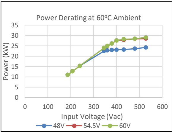
Figure 12: FCM30K Power Derating at 60°C
