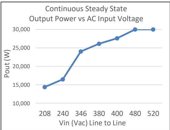
Figure 14: Steady State :FCM10K Output Power vs AC Input Voltage
