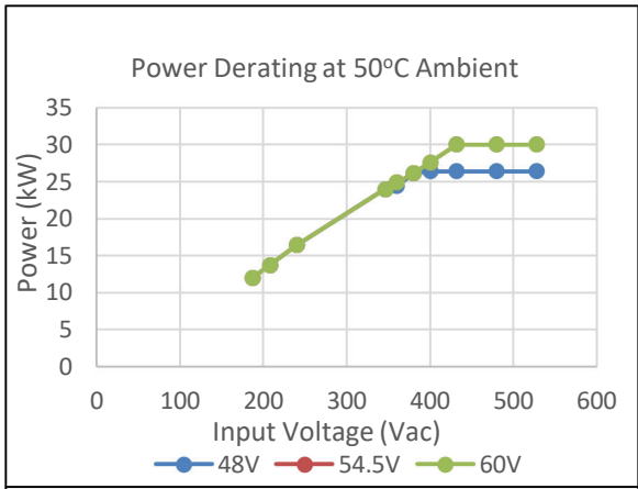
Figure 11: FCM30K Power Derating at 50°C
