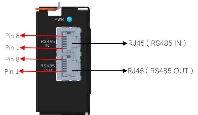
RJ45 Communication Signals Port
