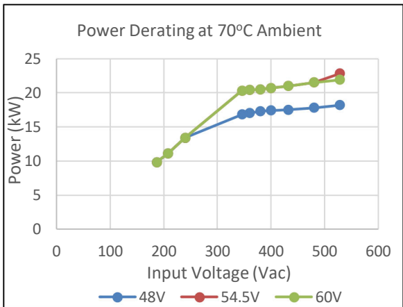
Figure 13: FCM30K Power Derating at 70°C
