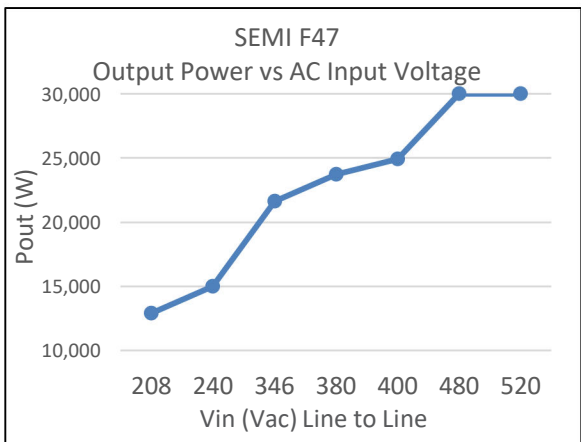
Figure 15: SEMI F47 : FCM30K Output Power vs AC Input Voltage
