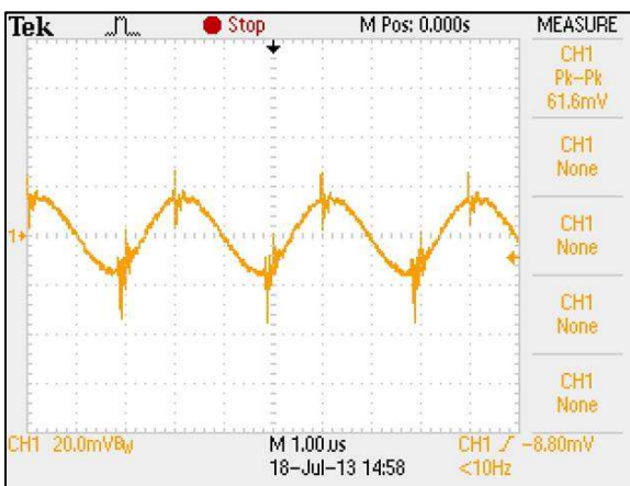
Figure 3: ERM10A72 Typical Output Ripple and Noise. Vin = 72Vdc Load: Io = 10A Ch 1: Vo
