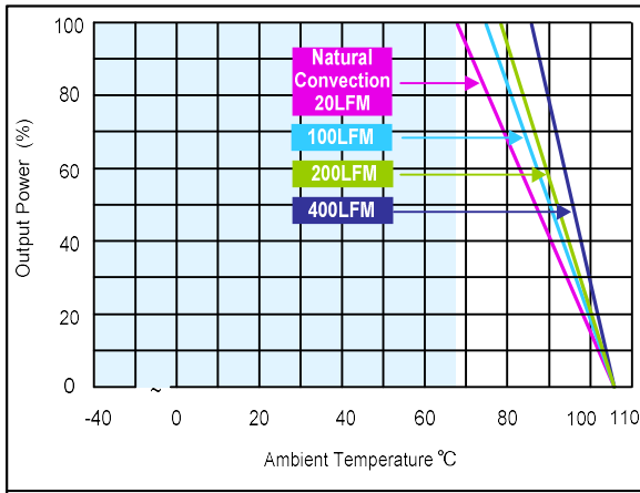
Figure 52: ERM04B110 Derating Curve without Heatsink Vin = 110Vdc Load: Io = 0 to 4.17A
