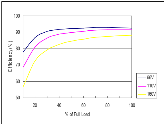
Figure 46: ERM04B110 Efficiency Versus Output Current Curve Vin = 66 to 160Vdc Load: Io = 0 to 4.17A
