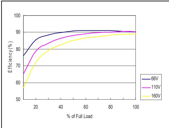
Figure 37: ERM10A110 Efficiency Versus Output Current Curve Vin = 66 to 160Vdc Load: Io = 0 to 10A
