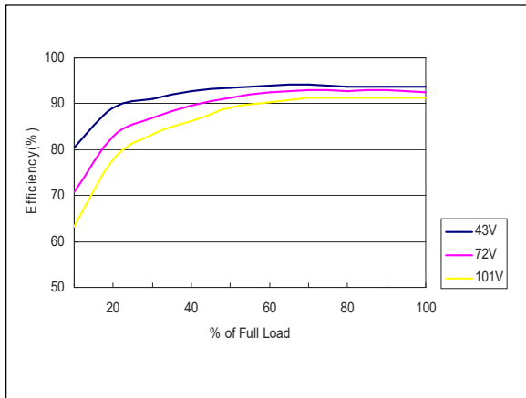
Figure 19: ERM03C72 Efficiency Versus Output Current Curve Vin = 43 to 101Vdc Load: Io = 0 to 3.33A
