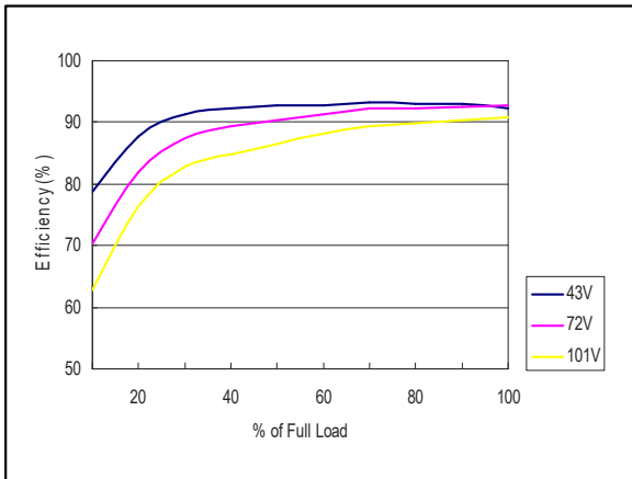
Figure 10: ERM04B72 Efficiency Versus Output Current Curve Vin = 43 to 101Vdc Load: Io = 0 to 4.17A
