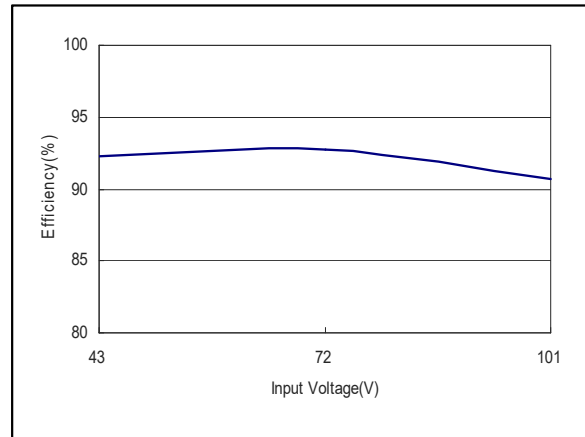
Figure 11: ERM04B72 Efficiency Versus Input Voltage Curve Vin = 43 to 101Vdc Load: Io = 0 to 4.17A
