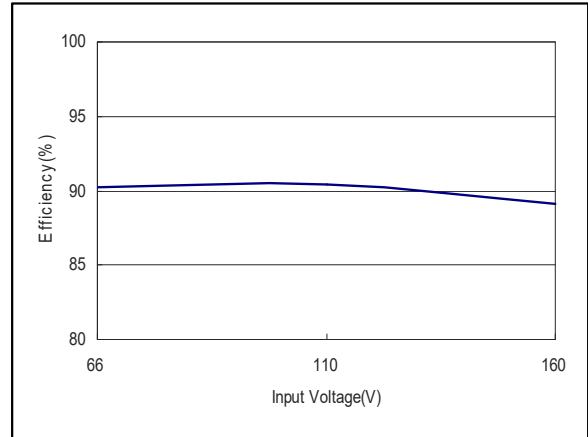
Figure 38: ERM10A110 Efficiency Versus Input Voltage Curve Vin = 66 to 160Vdc Load: Io = 0 to 10A
