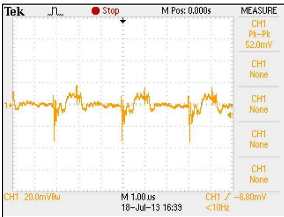
Figure 30: ERM02H72 Typical Output Ripple and Noise. Vin = 72Vdc Load: Io = 2.08A Ch 1: Vo
