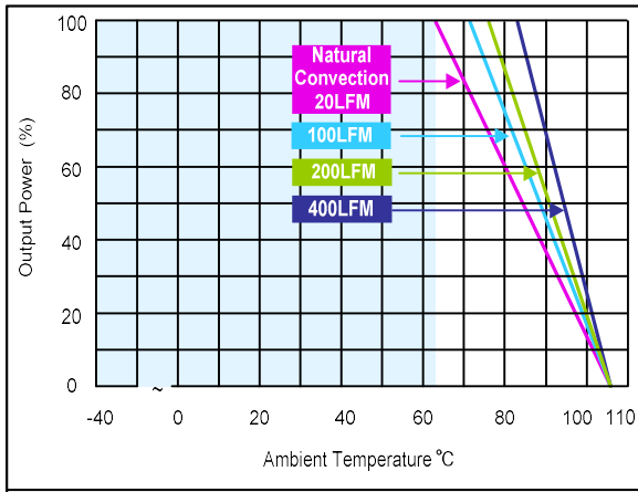
Figure 7: ERM10A72 Derating Curve without Heatsink Vin = 72Vdc Load: Io = 0 to 10A
