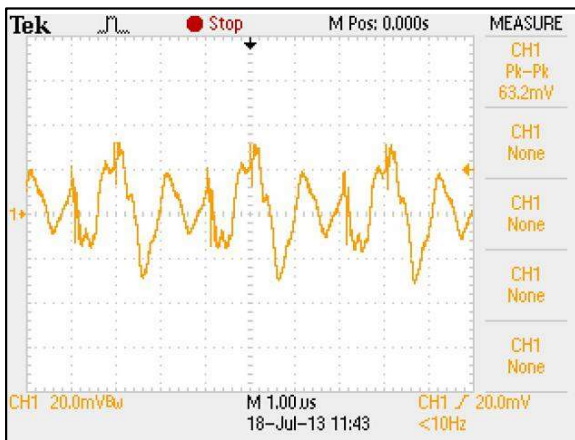
Figure 48: ERM04B110 Typical Output Ripple and Noise. Vin = 110Vdc Load: Io = 4.17A Ch 1: Vo
