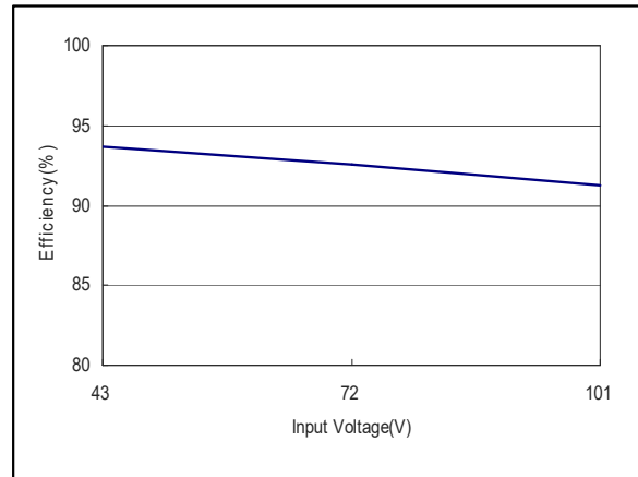
Figure 20: ERM03C72 Efficiency Versus Input Voltage Curve Vin = 43 to 101Vdc Load: Io = 0 to 3.33A
