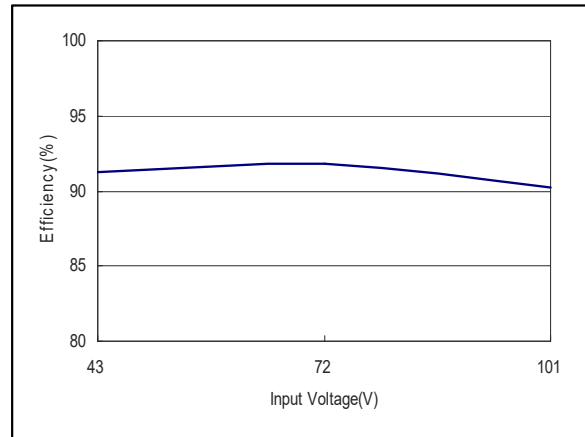
Figure 2: ERM10A72 Efficiency Versus Input Voltage Curve Vin = 43 to 101Vdc Load: Io = 0 to 10A
