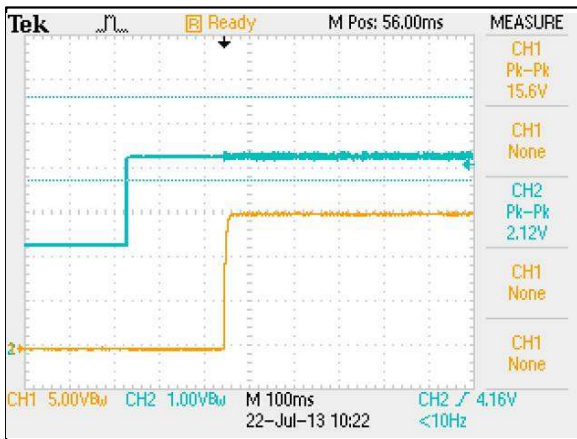
Figure 23: ERM03C72 Output Voltage Startup Characteristic by On/Off Vin = 72Vdc Load: Io = 3.33A Ch 1: Vo Ch 2: Remote On/Off
