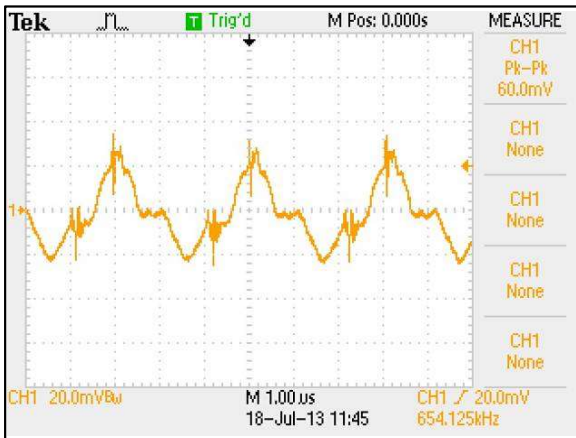
Figure 39: ERM10A110 Typical Output Ripple and Noise. Vin = 110Vdc Load: Io = 10A Ch 1: Vo
