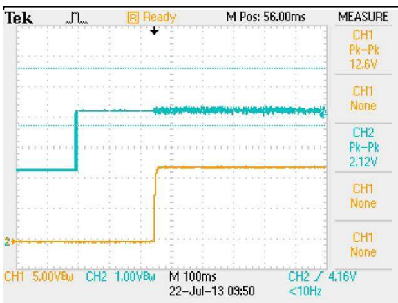
Figure 14: ERM04B72 Output Voltage Startup Characteristic by On/Off Vin = 72Vdc Load: Io = 4.17A Ch 1: Vo Ch 2: Remote On/Off
