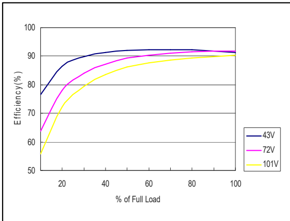
Figure 1: ERM10A72 Efficiency Versus Output Current Curve Vin = 43 to 101Vdc Load: Io = 0 to 10A
