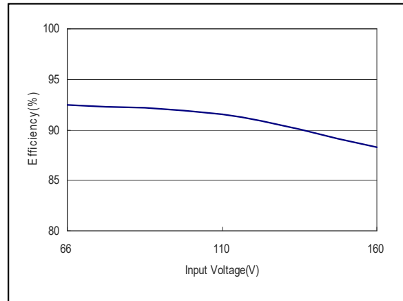
Figure 47: ERM04B110 Efficiency Versus Input Voltage Curve Vin = 66 to 160Vdc Load: Io = 0 to 4.17A
