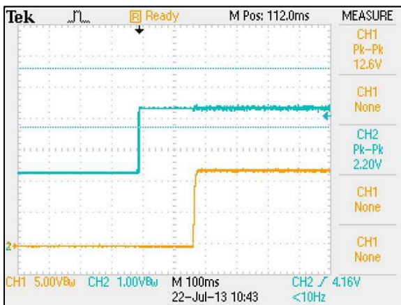
Figure 50: ERM04B110 Output Voltage Startup Characteristic by On/Off Vin = 110Vdc Load: Io = 4.17A Ch 1: Vo Ch 2: Remote On/Off
