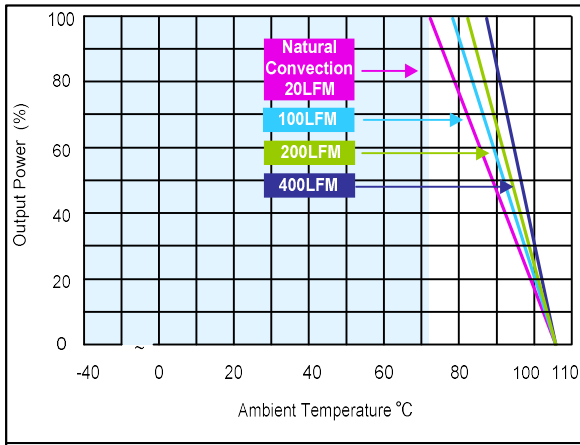
Figure 61: ERM03C110 Derating Curve without Heatsink Vin = 110Vdc Load: Io = 0 to 3.33A
