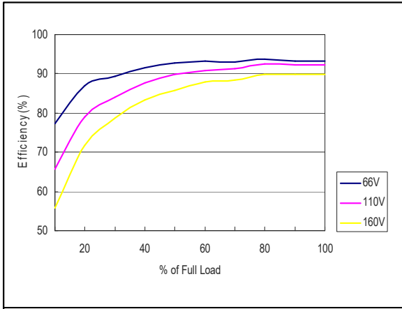
Figure 55: ERM03C110 Efficiency Versus Output Current Curve Vin = 66 to 160Vdc Load: Io = 0 to 3.33A
