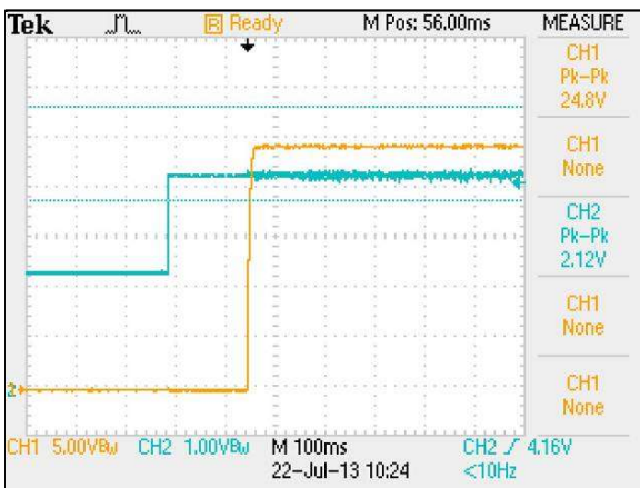
Figure 32: ERM02H72 Output Voltage Startup Characteristic by On/Off Vin = 72Vdc Load: Io = 2.08A Ch 1: Vo Ch 2: Remote On/Off
