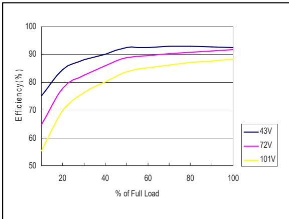
Figure 28: ERM02H72 Efficiency Versus Output Current Curve Vin = 43 to 101Vdc Load: Io = 0 to 2.08A
