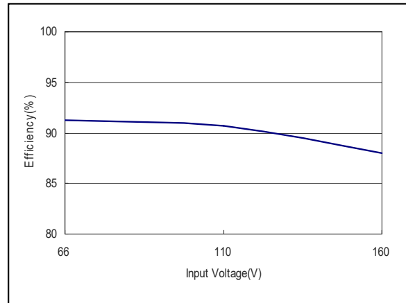
Figure 65: ERM02H110 Efficiency Versus Input Voltage Curve Vin = 66 to 160Vdc Load: Io = 0 to 2.08A
