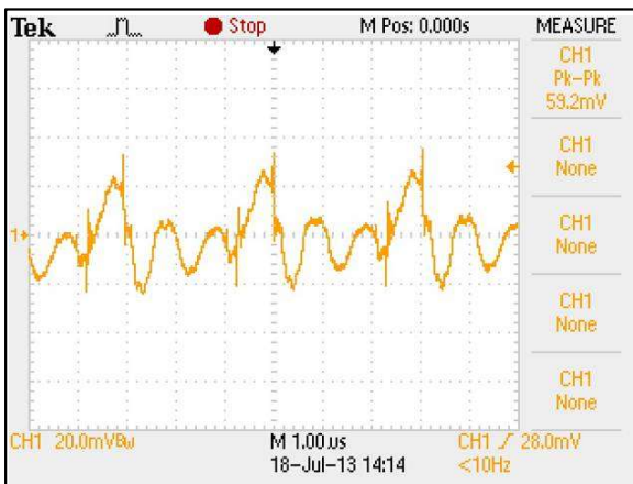
Figure 66: ERM02H110 Typical Output Ripple and Noise. Vin = 110Vdc Load: Io = 2.08A Ch 1: Vo
