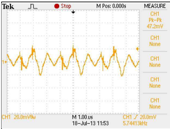
Figure 57: ERM03C110 Typical Output Ripple and Noise. Vin = 110Vdc Load: Io = 3.33A Ch 1: Vo
