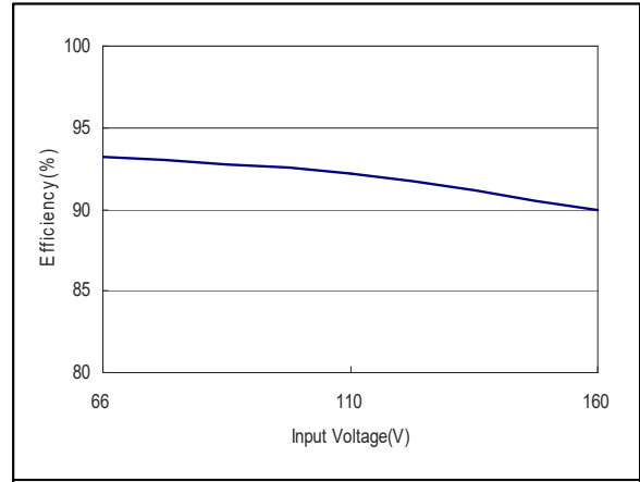
Figure 56: ERM03C110 Efficiency Versus Input Voltage Curve Vin = 66 to 160Vdc Load: Io = 0 to 3.33A
