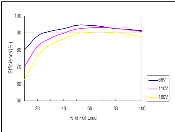
Figure 64: ERM02H110 Efficiency Versus Output Current Curve Vin = 66 to 160Vdc Load: Io = 0 to 2.08A
