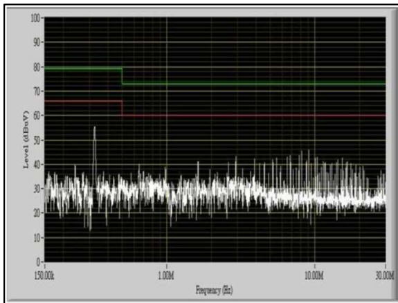
Figure 63: ERM03C110 Conduction Emission of EN55011 Class A Vin = 110Vdc Load: Io = 3.33A
