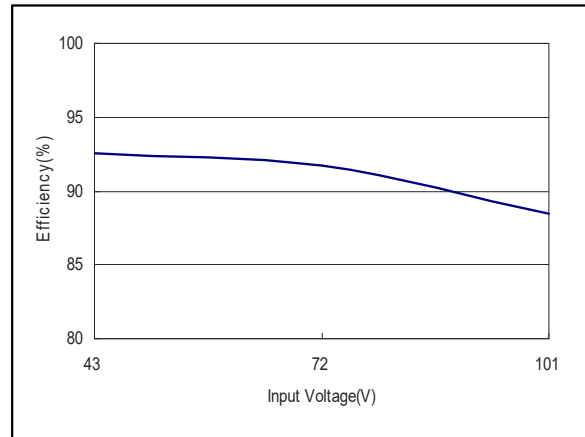
Figure 29: ERM02H72 Efficiency Versus Input Voltage Curve Vin = 43 to 101Vdc Load: Io = 0 to 2.08A
