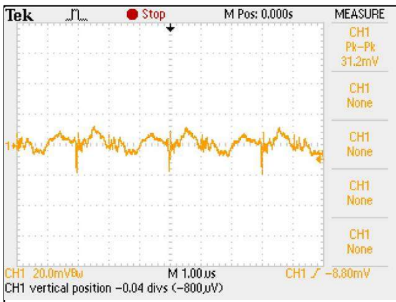
Figure 21: ERM03C72 Typical Output Ripple and Noise. Vin = 72Vdc Load: Io = 3.33A Ch 1: Vo
