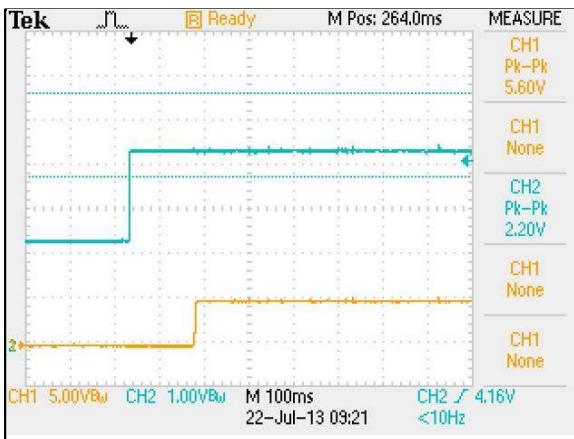
Figure 5: ERM10A72 Output Voltage Startup Characteristic by On/Off Vin = 72Vdc Load: Io = 10A Ch 1: Vo Ch 2: Remote On/Off
