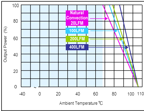
Figure 34: ERM02H72 Derating Curve without Heatsink Vin = 72Vdc Load: Io = 0 to 2.08A
