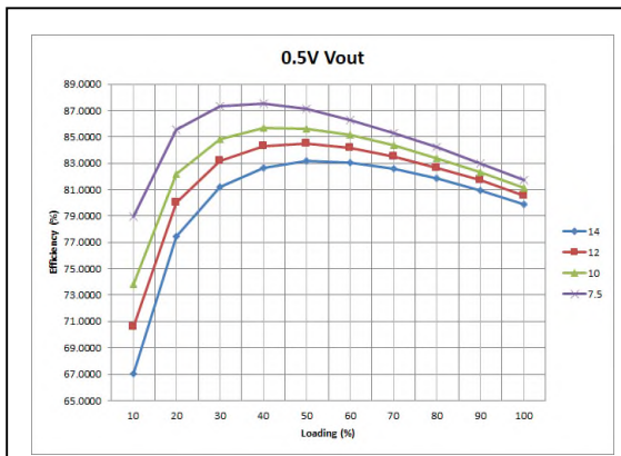
Figure 1: LGA110D-00DADJJB Efficiency Curves at different V_{IN} @ 25°C Loading: I_O = 10% increment to 110A, V_O = 0.5V Frequency=533KHz
