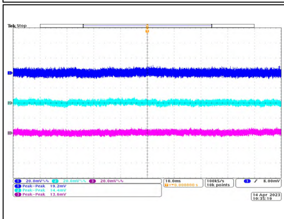
Figure 22: LGA110D-01DADJJB Ripple and Noise - V_o = 3.3V Full Load Ch 1: V_{O1} Ch 2: V_{O2} Ch 3: V_{O3}
