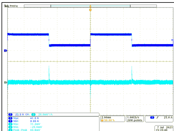
Figure 32: LGA110D-01DADJJB Transient Response - Vo Deviation 25% to 75% to 25% load change, 1A/ \mu S slew rate, Vin = 12Vdc Vo = 1.8V Ch 1: I O Ch 2: V O F SW =533kHz
