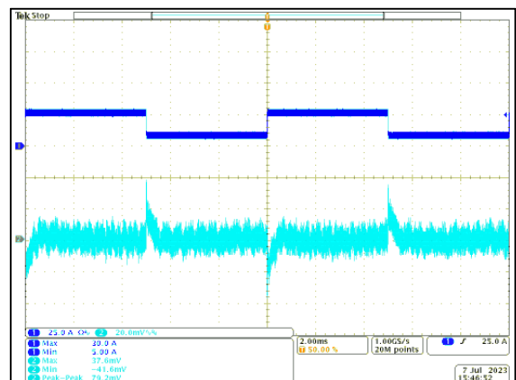
Figure 35: LGA110D-01DADJJB Transient Response - Vo Deviation 25% to 75% to 25% load change, 1A/ \mu S slew rate, Vin = 12Vdc Vo = 5.0V Ch 1: I O Ch 2: V O F SW =533kHz
