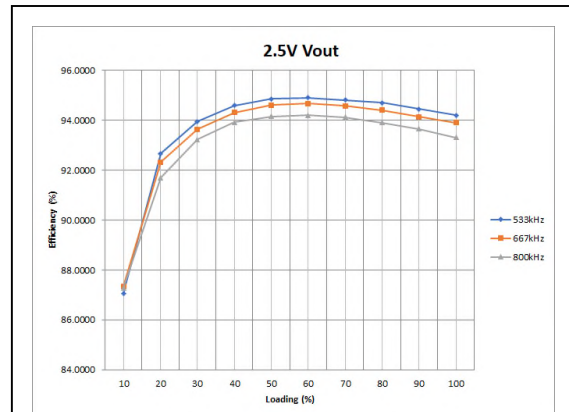
Figure 10: LGA110D-01DADJJB Efficiency Curves at different switching frequency @ 25°C, Vin = 12V Loading: I O = 10% increment to 90A
