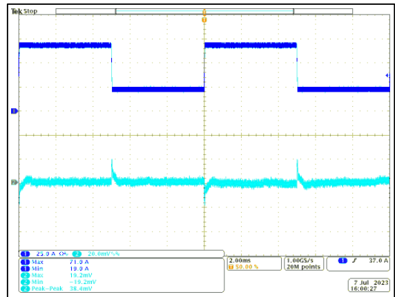
Figure 39: LGA110D-01DADJJB Transient Response - Vo Deviation 25% to 75% to 25% load change, 1A/ \mu S slew rate, Vin = 12Vdc Vo = 2.5V Ch 1: Io Ch 2: Vo F SW =533kHz
