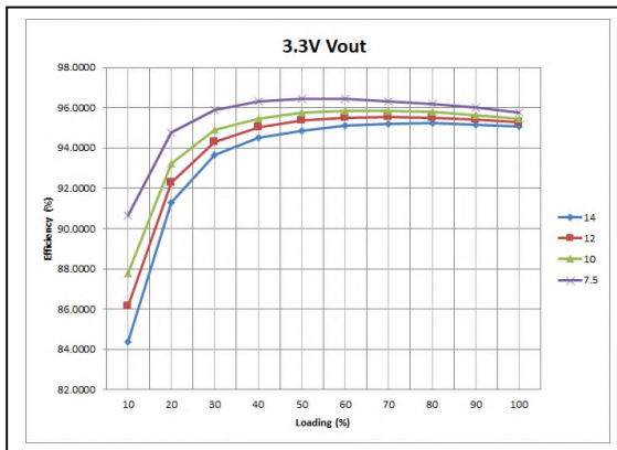
Figure 5: LGA110D-01DADJJB Efficiency Curves at different V_{IN} @ 25°C Loading: I_O = 10% increment to 80A, V_O = 3.3V Frequency=533KHz
