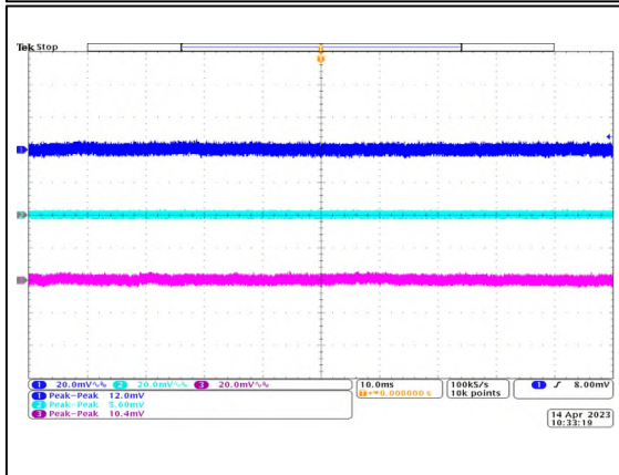
Figure 20: LGA110D-01DADJJB Ripple and Noise - V_o = 1.8V Full Load Ch 1: V_{O1} Ch 2: V_{O2} Ch 3: V_{O3}
