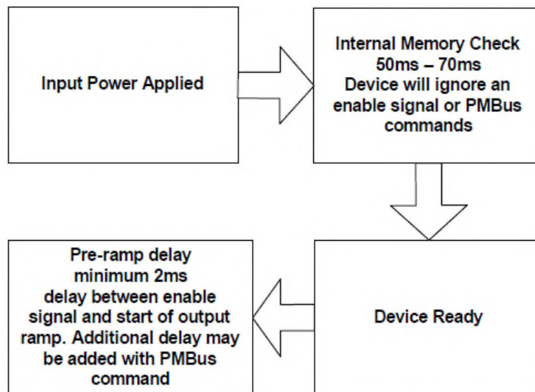
Figure 61: Start-Up Procedure
