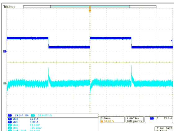
Figure 34: LGA110D-01DADJJB Transient Response - Vo Deviation 25% to 75% to 25% load change, 1A/ \mu S slew rate, Vin = 12Vdc Vo = 3.3V Ch 1: I O Ch 2: V O F SW =533kHz
