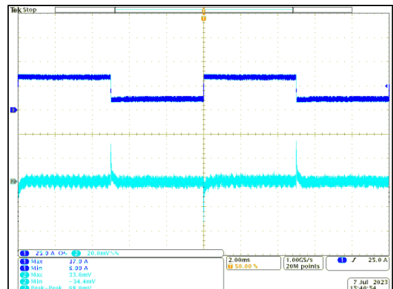
Figure 33: LGA110D-01DADJJB Transient Response - Vo Deviation 25% to 75% to 25% load change, 1A/ \mu S slew rate, Vin = 12Vdc Vo = 2.5V Ch 1: I O Ch 2: V O F SW =533kHz
