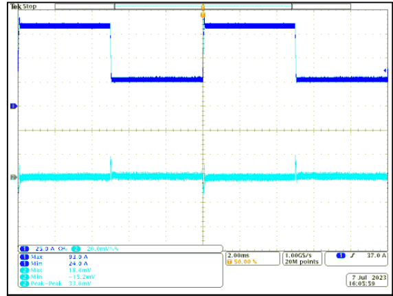
Figure 37: LGA110D-01DADJJB Transient Response - Vo Deviation 25% to 75% to 25% load change, 1A/ \mu S slew rate, Vin = 12Vdc Vo = 1.0V Ch 1: Io Ch 2: Vo F SW =533kHz
