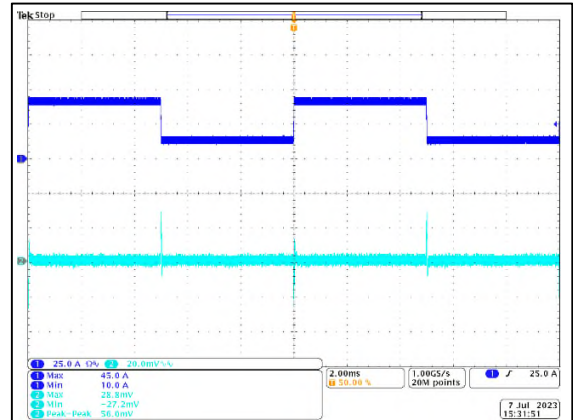
Figure 31: LGA110D-01DADJJB Transient Response - Vo Deviation 25% to 75% to 25% load change, 1A/ \mu S slew rate, Vin = 12Vdc Vo = 1.0V Ch 1: I O Ch 2: V O F SW =533kHz
