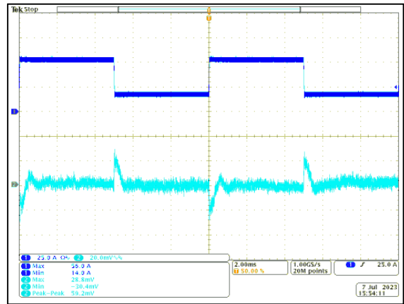
Figure 41: LGA110D-01DADJJB Transient Response - Vo Deviation 25% to 75% to 25% load change, 1A/ \mu S slew rate, Vin = 12Vdc Vo = 5.0V Ch 1: Io Ch 2: Vo F SW =533kHz
