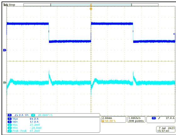
Figure 40: LGA110D-01DADJJB Transient Response - Vo Deviation 25% to 75% to 25% load change, 1A/ \mu S slew rate, Vin = 12Vdc Vo = 3.3V Ch 1: Io Ch 2: Vo F SW =533kHz
