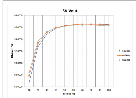
Figure 12: LGA110D-01DADJJB Efficiency Curves at different switching frequency @ 25°C, Vin = 12V Loading: I O = 10% increment to 70A
