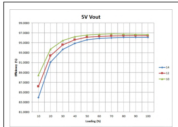
Figure 6: LGA110D-00DADJJB Efficiency Curves at different V_{IN} @ 25°C Loading: I_O = 10% increment to 70A, V_O = 5V Frequency=533KHz
