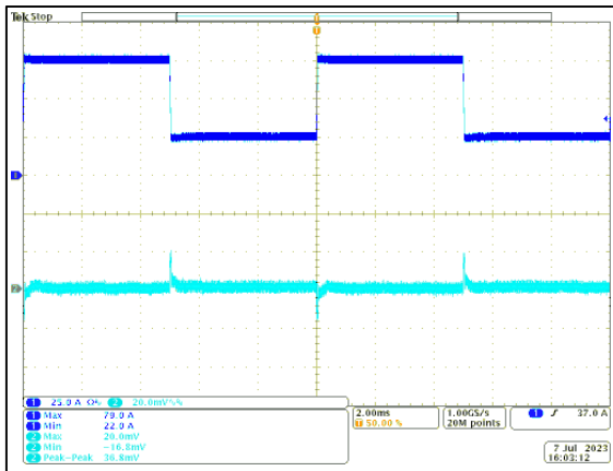
Figure 38: LGA110D-01DADJJB Transient Response - Vo Deviation 25% to 75% to 25% load change, 1A/ \mu S slew rate, Vin = 12Vdc Vo = 1.8V Ch 1: Io Ch 2: Vo F SW =533kHz
