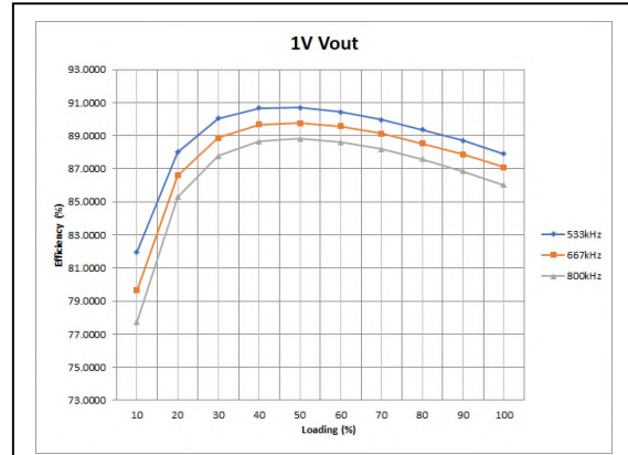
Figure 8: LGA110D-01DADJJB Efficiency Curves at different switching frequency @ 25°C, Vin = 12V Loading: I O = 10% increment to 110A
