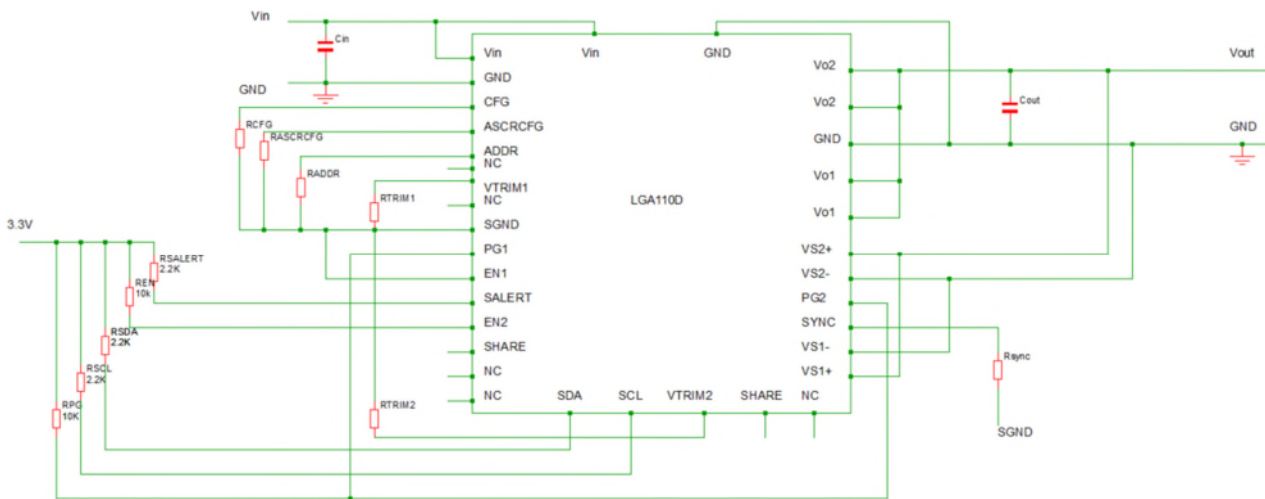
Figure 57: One module one output
