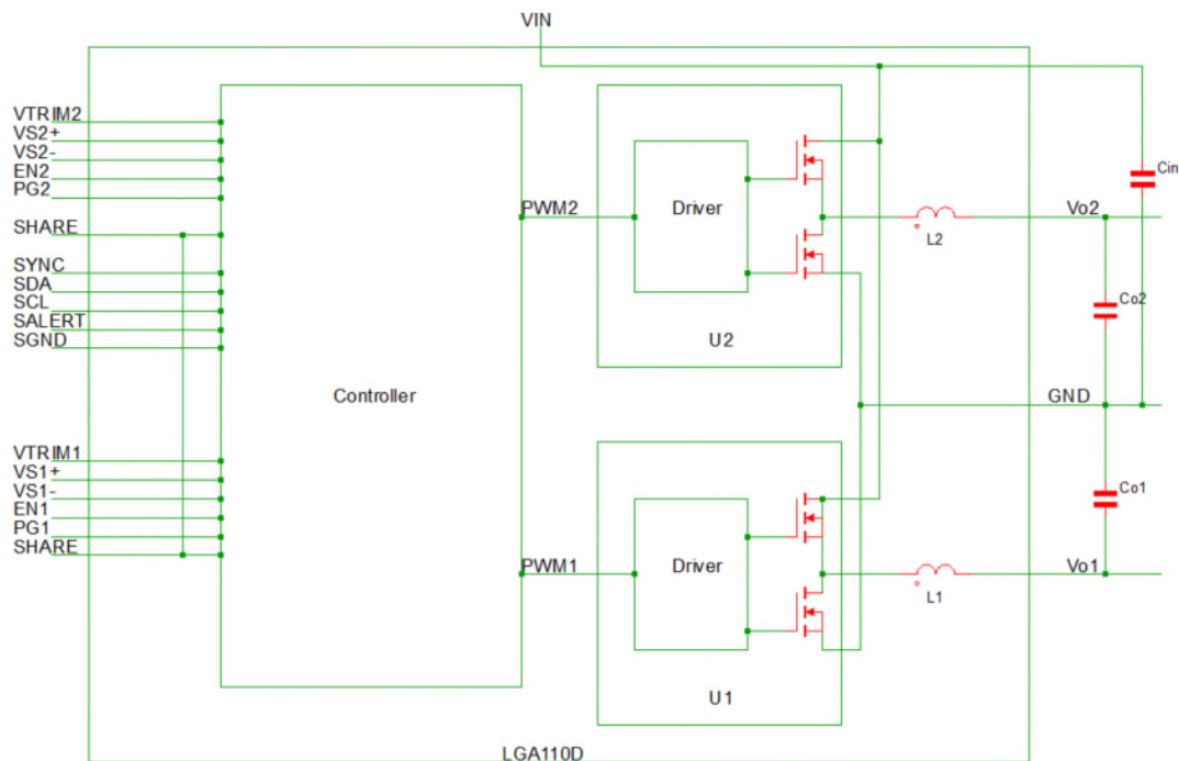
Figure 55: Electrical Block Diagram
