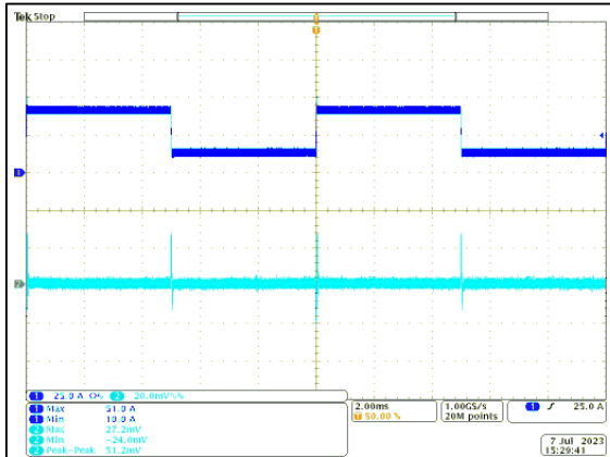
Figure 30: LGA110D-01DADJJB Transient Response - Vo Deviation 25% to 75% to 25% load change, 1A/ \mu S slew rate, Vin = 12Vdc Vo = 0.5V Ch 1: I O Ch 2: V O F SW =533kHz
