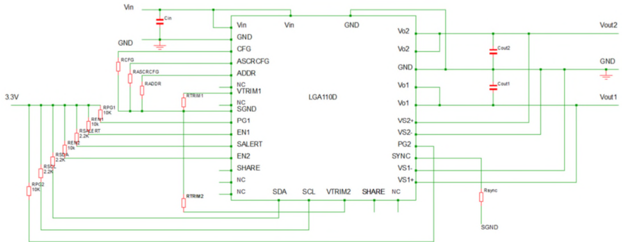
Figure 56: Standard Application (dual output)
