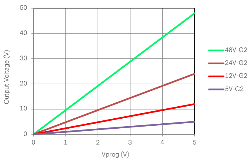
Figure 55 Example of Vprog vs. output Voltage
