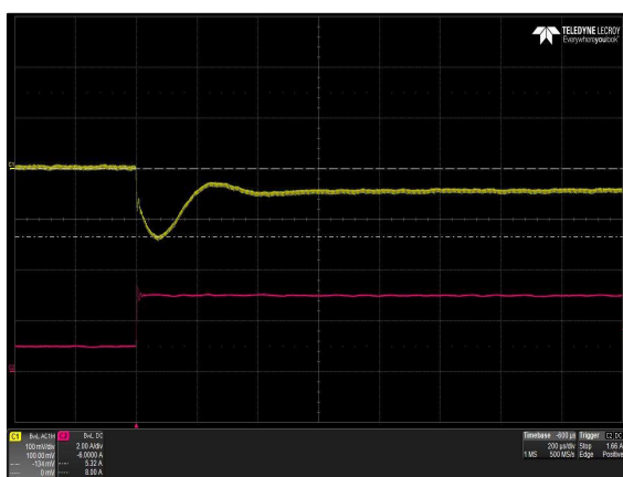
Figure 53: \mu MP16T-ILL-00-A Transient Response - V_O Deviation 25% to 75% load change, 1A/ \mu S slew rate, C_O = 470\mu F Ch 1: V_{O1} Ch 2: I_{O1}
