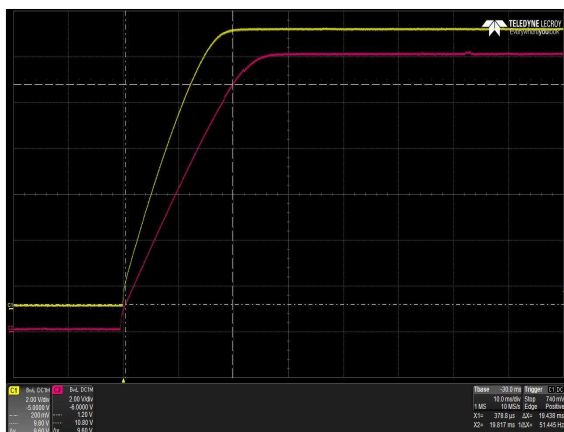
Figure 51: \mu MP16T-ILL-00-A Output Voltage Startup Characteristic Load: I_{O1} = 4A , I_{O2} = 4A Ch 1: V_{O1} Ch 2: V_{O2}
