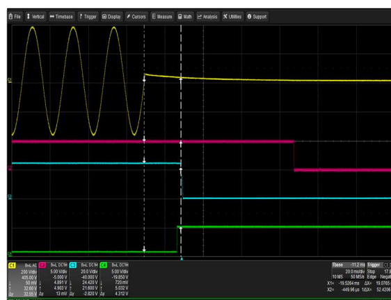
Figure 22: μMP10T-S2Q-S2Q-S2Q-S2Q-S2Q-90-A Hold-up Time via AC mains V_{in} = 264V_{ac}/47Hz Load: I_O = 50A I_{SB} = 2A Ch 1: AC Mains Ch 2: V_{SB} Ch 3: V_O Ch 4: Global DCOK
