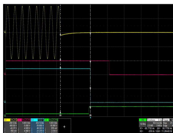
Figure 24: μMP10T-S2W-HUP-00-A Hold-up Time V_{in} = 264V_{ac}/47Hz Load: I_O = 5A I_{SB} = 2A Ch 1: AC Mains Ch 2: V_{SB} Ch 3: V_O Ch 4: Global DCOK
