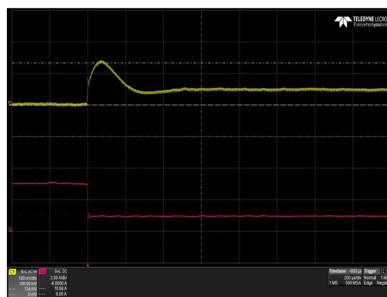
Figure 54: \mu MP16T-ILL-00-A Transient Response - V_O Deviation 75% to 25% load change, 1A/ \mu S slew rate, C_O = 470\mu F Ch 1: V_{O1} Ch 2: I_{O1}
