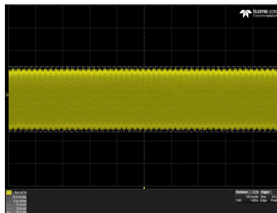
Figure 52: \mu MP16T-ILL-00-A Ripple and Noise Measurement Load: I_{O1} = 4A Ch 1: V_{O1}
