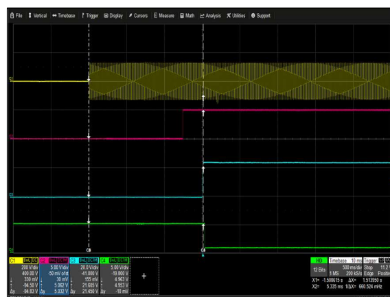
Figure 19: μMP10T-S2Q-S2Q-S2Q-S2Q-S2Q-90-A Turn-on delay via AC mains V_{in} = 90V_{ac} Load: I_O = 41.66A I_{SB} = 2A Ch 1: AC Mains Ch 2: V_{SB} Ch 3: V_O Ch 4: Global DCOK
