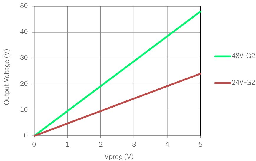
Figure 56 Example of Vprog vs. output Voltage
