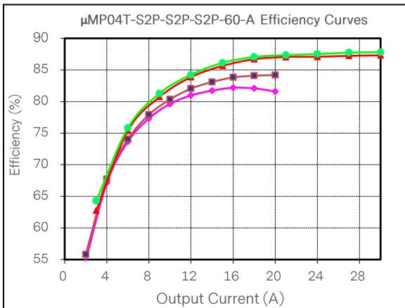
Figure 9: μMP04T-S2P-S2P-S2P-60-A Efficiency Curve @ 25°C * 90Vac * 115Vac * 230Vac * 264Vac Loading: I_{o\_main} = 10\%I_{o\_max} increment to 30A, I_{SB} = 0A
