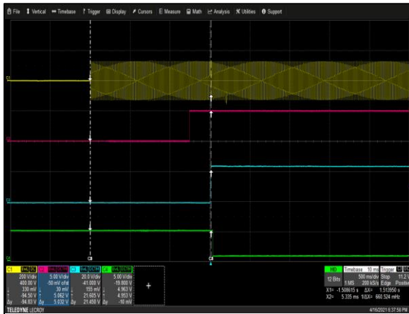
Figure 19: µMP10T-S2Q-S2Q-S2Q-S2Q-S2Q-S2Q-90-A Turn-on delay via AC mains Vin = 90Vac Load: I O = 41.66A I SB = 2A Ch 1: AC Mains Ch 2: V SB Ch 3: V O Ch 4: Global DCOK
