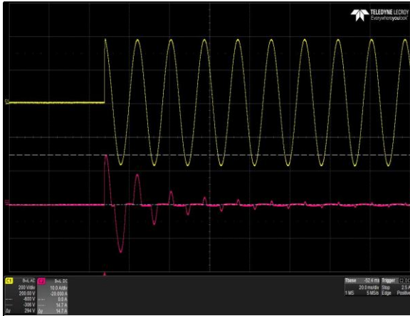
Figure 7: μMP04T-S2P-S2P-S2P-60-A Start up Inrush Current Vin = 264Vac Load: I_o = 0A I_{SB} = 0A Turn On Phase = 90^\circ Ch 1: V_N Ch 2: I_N
