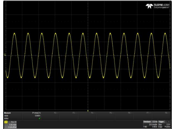
Figure 8: μMP04T-S2P-S2P-S2P-60-A Input Current Waveform Vin = 90Vac Load: I_o = 20A I_{SB} = 1A Ch 1: I_N
