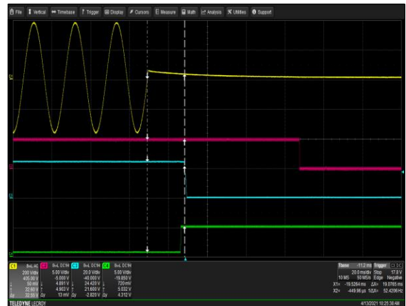
Figure 22: µMP10T-S2Q-S2Q-S2Q-S2Q-S2Q-S2Q-90-A Hold-up Time via AC mains Vin = 264Vac/47Hz Load: I O = 50A I SB = 2A Ch 1: AC Mains Ch 2: V SB Ch 3: V O Ch 4: Global DCOK
