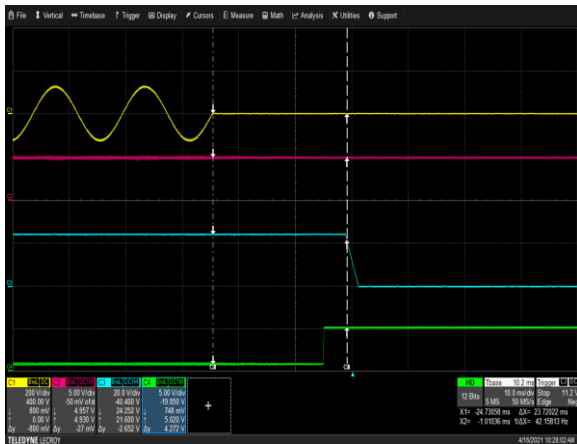
Figure 32: μMP16C-SKQ-SKQ-30-A Hold-up Time Vin = 90Vac/63Hz Load: I o = 41.66A I SB = 2A Ch 1: AC Mains Ch 2: V SB Ch 3: V O Ch 4: Global DCOK
