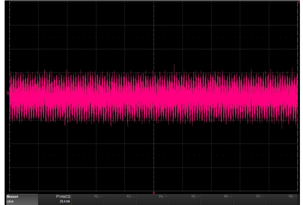
Figure 38: iHP24H3A-S1-00 Ripple and Noise Measurement Load: R = 2.13 ohm Ch 2: I_o
