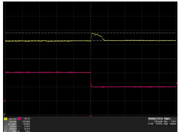
Figure 18: iHP24H3A-S2-00 Transient Response - V_o Deviation 100% to 50% load change, 0.5A/\mu S slew rate Ch 1: V_o Ch 2: I_o
