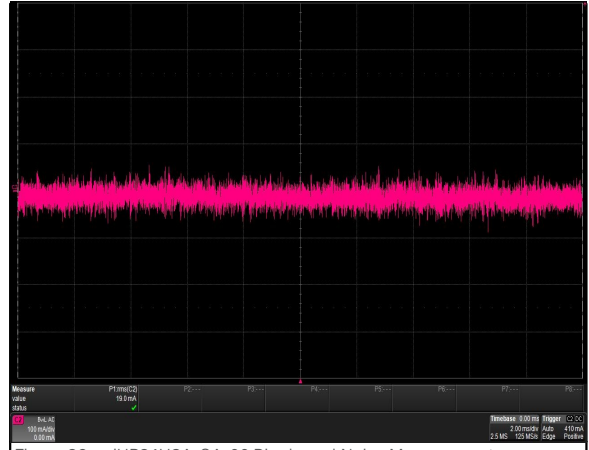
Figure 26: iHP24H3A-SA-00 Ripple and Noise Measurement Load: R = 13.3 ohm Ch 2: I_o
