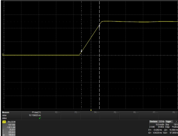
Figure 15: iHP24H3A-S2-00 Output Voltage Startup Characteristic Load: I_o = 12A Ch 1: V_o
