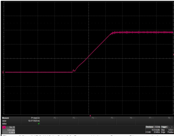
Figure 25: iHP24H3A-SA-00 Output Voltage Startup Characteristic Load: R = 13.3 ohm Ch 2: I_o
