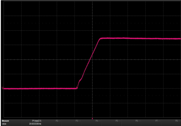
Figure 37: iHP24H3A-S1-00 Output Voltage Startup Characteristic Load: R = 2.13 ohm Ch 2: I_o
