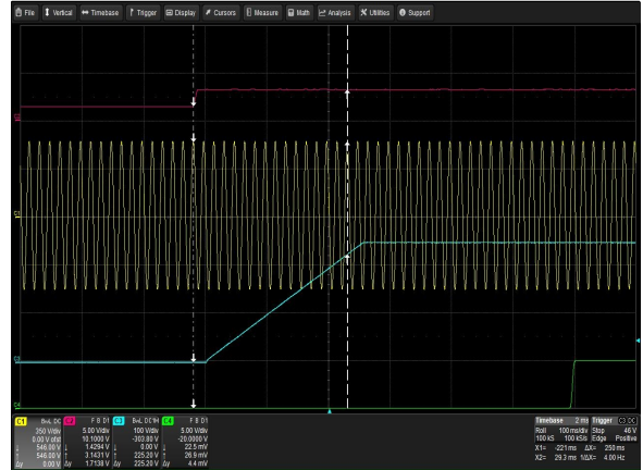
Figure 2: iHP24H3A-S2-00 Turn-on delay via Global inhibit Vin = 380Vac Load: I_o = 12A I_{SB} = 1A Ch 1: AC Mains Ch 2: Global inhibit Ch 3: V_o Ch 4: Global DCOK
