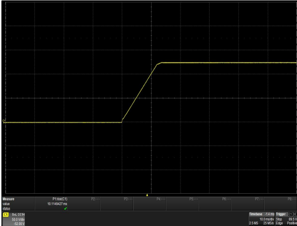
Figure 27: iHP24H3A-S1-00 Output Voltage Startup Characteristic Load: I_o = 12A Ch 1: V_o
