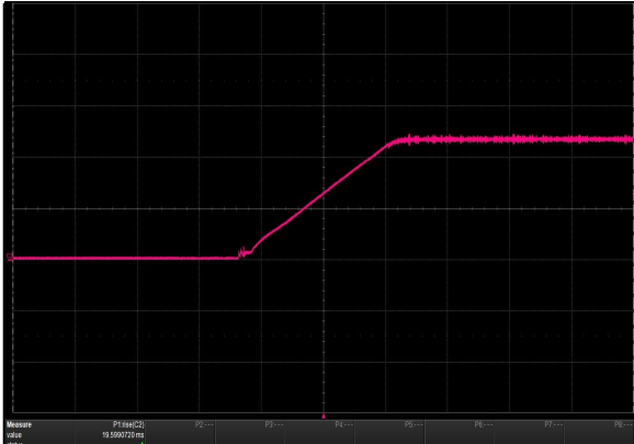
Figure 19: iHP24H3A-S2-00 Output Voltage Startup Characteristic Load: R = 20.8 ohm Ch 2: I_o
