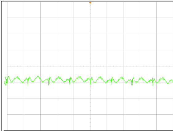
Figure 1: ADH1300-48S28B Input Reflected Ripple Current Vin = 48Vdc Load: Io = 46.5A Ch 2: Iin (5uS/div, 50mV/div)
