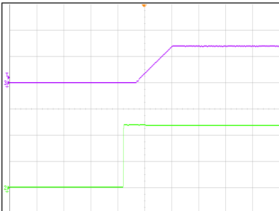
Figure 3: ADH1300-48S28B Output Voltage Startup Characteristic Vin = 48Vdc Load: Io = 46.5A (100mS/div) Ch 2: Vi (20V/div) Ch 3: Vo (20V/div)
