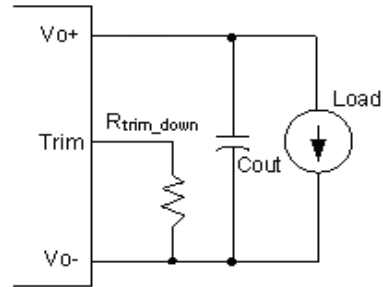
Figure 17 Trim down
