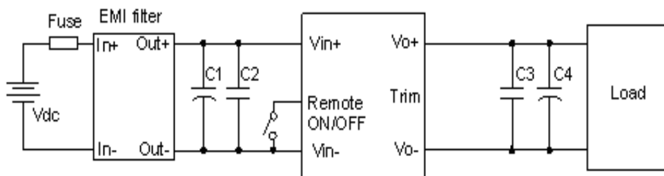
Figure 14 Typical application
