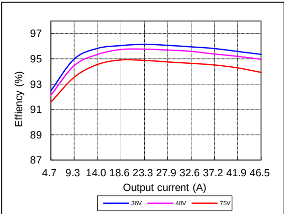
Figure 9: ADH1300-48S28B Efficiency Curves Vin = 36 to 75Vdc Loading: Io = 5A to 46.5A
