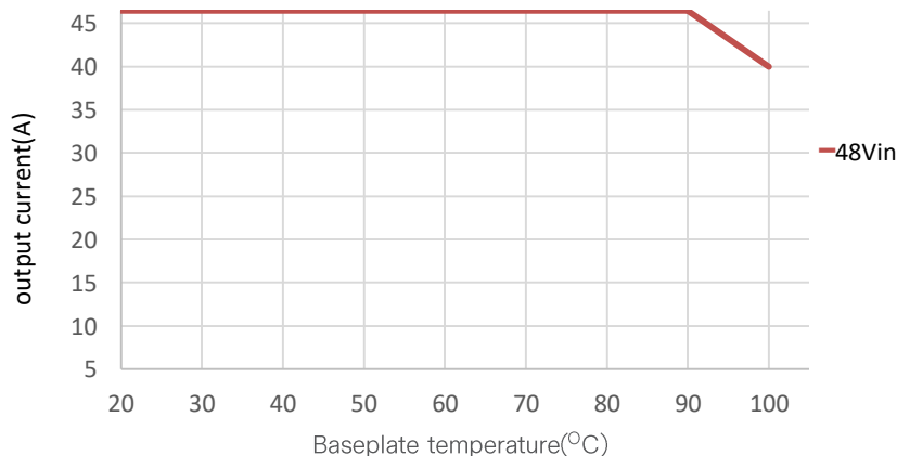
Figure 13 Available load current vs Base plate temperature
