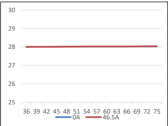
Figure 10: ADH1300-48S28B Output voltage vs. input voltage and load current at T = +25°C
