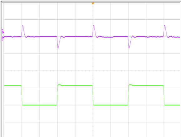
Figure 7: ADH1300-48S28B Transient Response (2mS/div) Vin = 48Vdc Io = 50%-75%~50% load change, 0.1A/uS slew rate Ch 2: Io (10A/div) Ch 3: Vo (500mV/div)
