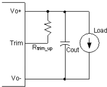
Figure 16 Trim up
