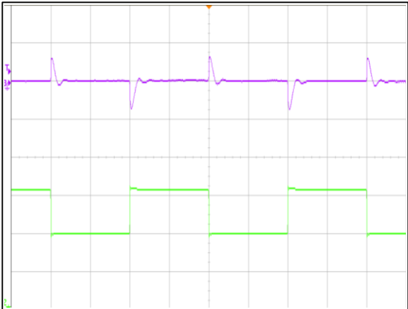
Figure 8: ADH1300-48S28B Transient Response (2mS/div) Vin = 48Vdc Io = 25%-50%~25% load change, 0.1A/uS slew rate Ch 2: Io (10A/div) Ch 3: Vo (500mV/div)
