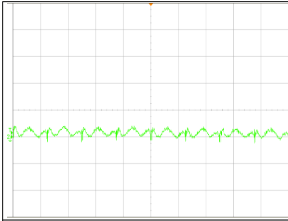
Figure 1: ADH1300-48S28B Input Reflected Ripple Current V_{in} = 48V_{dc} Load: I_o = 46.5A Ch 2: I_{in} (5uS/div, 50mV/div)
