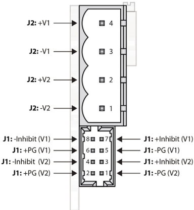
CmG & CmH Output Connectors
