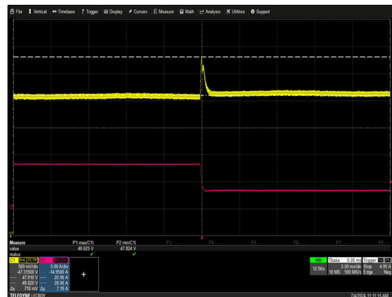
Figure 54: NP08W1-1MW0-00-A-0 Transient Response - V_O Deviation 100% to 40% load change, 1A/μs slew rate Ch 1: V_O Ch 2: I_O
