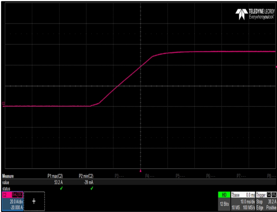
Figure 21: NP08W1-1ME0-00-A-0 Output Current Startup Characteristic Load: R = 0.08 ohm Ch 2: I_O
