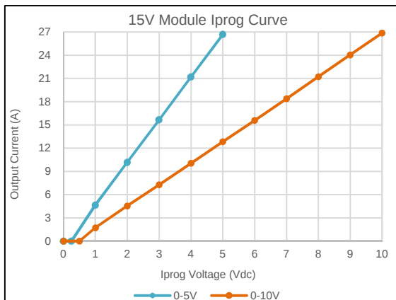
Figure 41: NP08W1-1MN0-00-A-0 Output Current Adjustment @ 25°C
