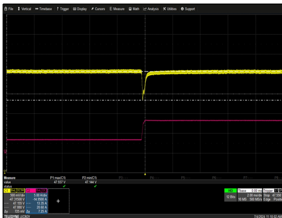
Figure 53: NP08W1-1MW0-00-A-0 Transient Response - V_O Deviation 40% to 100% load change, 1A/μs slew rate Ch 1: V_O Ch 2: I_O
