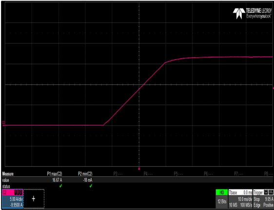
Figure 48: NP08W1-1MQ0-00-A-0 Output Current Startup Characteristic Load: R = 1.43 ohm Ch 2: I_O
