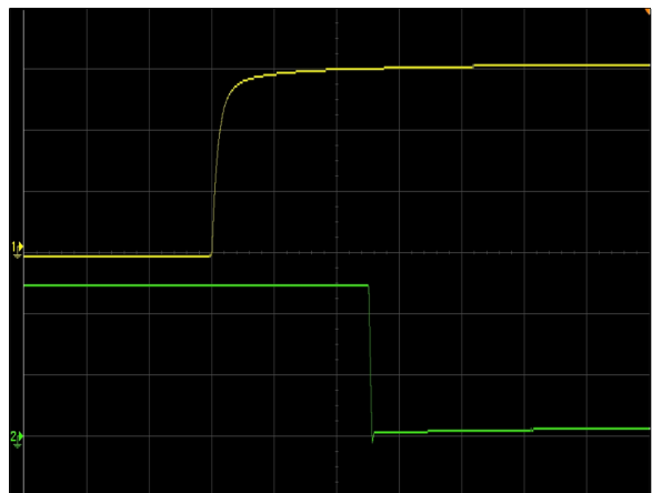
Figure 4: NDQ1300-48S12B-6LI Remote Off Waveform (10ms/div) Vin = 50V Load: Io = 106A Ch 1: Remote Off (1V/div) Ch 2: Vo (5V/div)
