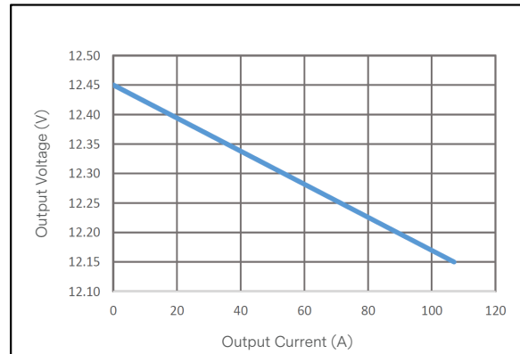
Figure 8: NDQ1300-48S12B-6LI Output Voltage vs. Output Current
