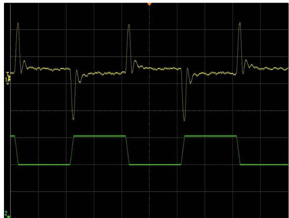
Figure 6: NDQ1300-48S12B-6LI Transient Response (2ms/div) Vin = 50V Io = 25% load step, 50%-75%-50%, 0.1A/μs slew rate Ch 1: Vo (100mV/div) Ch 2: Io (25A/div)
