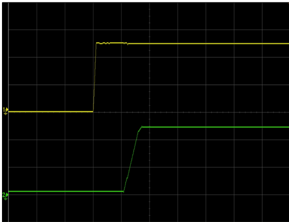
Figure 1: NDQ1300-48S12B-6LI Output Voltage Startup (50ms/div) Vin = 50V Load: Io = 106A Ch1: Vin (20V/div) Ch2: Vo (5V/div)
