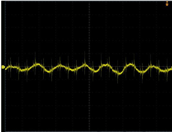
Figure 7: NDQ1300-48S12B-6LI Input Reflected Ripple Current V_{in} = 50V Load: I_o = 106A Ch 1: I_{in} ( 5\mu s/div , 100mA/div )
