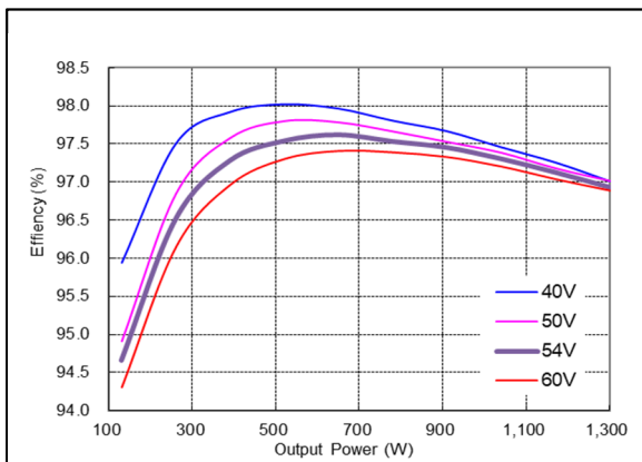
Figure 9: NDQ1300-48S12B-6LI Efficiency Curves
