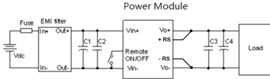
Figure 13 Typical application
