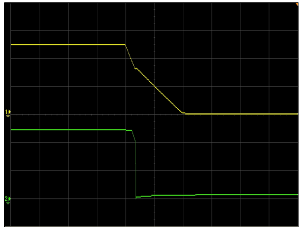
Figure 2: NDQ1300-48S12B-6LI Turn Off Characteristic (50ms/div) Vin = 50V Load: Io = 106A Ch1: Vin (20V/div) Ch2: Vo (5V/div)
