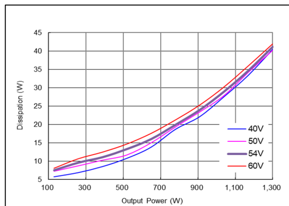
Figure 10: NDQ1300-48S12B-6LI Power Loss vs. Output Power
