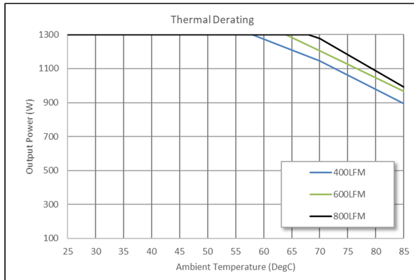
Figure 12 NDQ1300-48S12B-6LI with 0.7" heatsink, output power derating at 50Vin, air flowing across the converter from Vin- to Vin+
