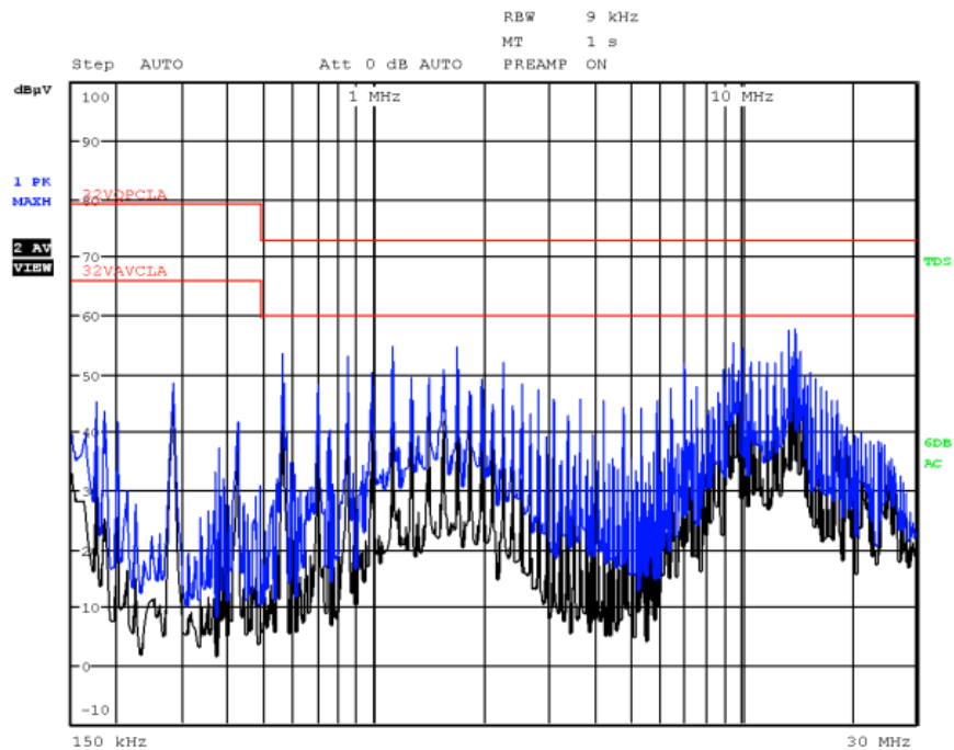
Figure 17: Conducted Emissions (2 AIF06ZPFC series modules)
