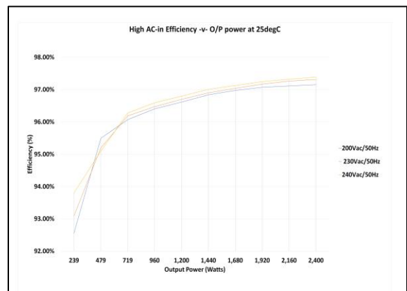
Figure 12: AIF06ZPFC Efficiency Curve @ 25°C — 230VAC — 200VAC — 240VDC Loading: P_{O,max} = 2400W 10% increment to P_{O,max}
