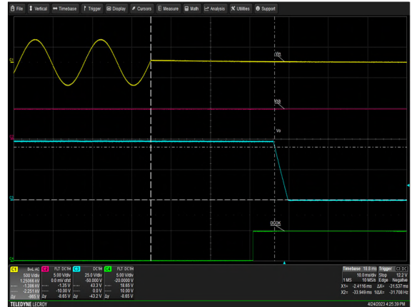
Figure 18: LCC1200-48U-9P Hold-up Time Vin = 264Vac Load: Io = 25A (48V), I SB = 1.5A (5V) Ch 1: AC Mains Ch 2: V SB Ch 3: V O CH 4: G_DCOK_C
