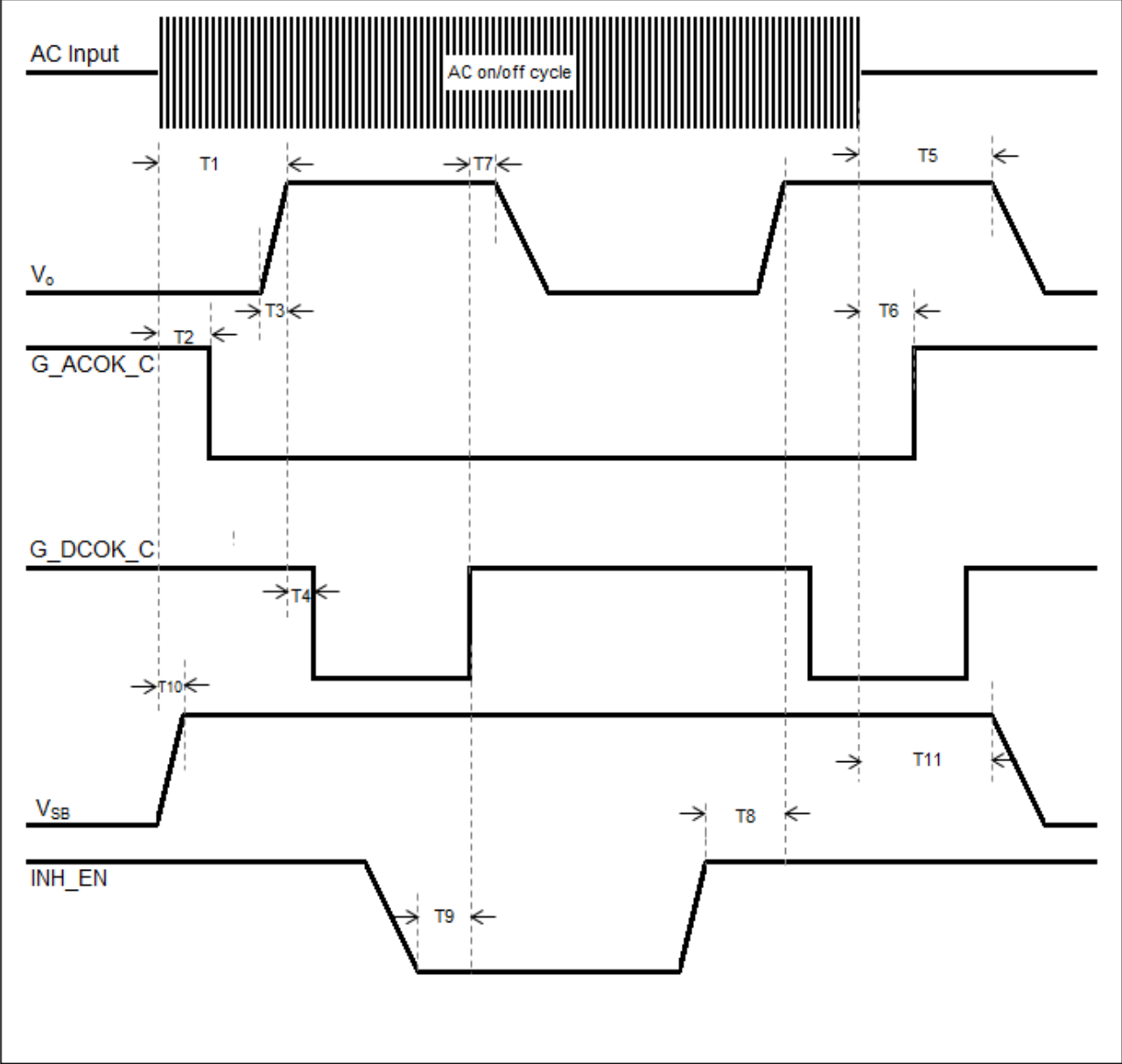
System Timing Diagram
