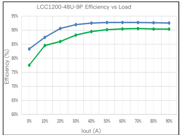
Figure 24: LCC1200-48U-9P Efficiency Curve @ 25°C Loading: I o,max = 10% I o,max increment to full load
