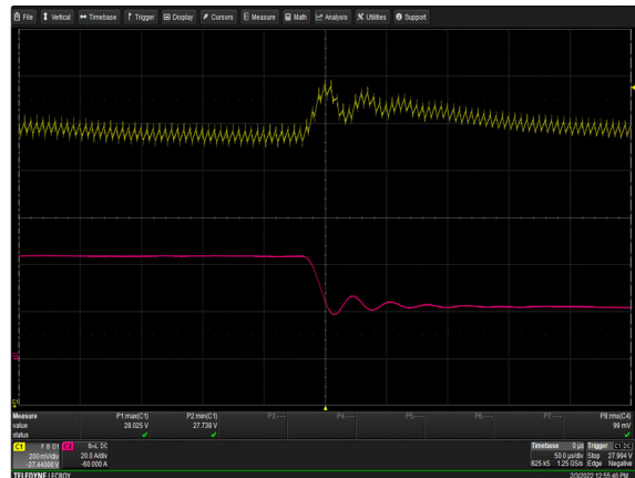
Figure 10: LCC1200-28U-9P Transient Response - V_o Deviation 100% to 50% load change (1KHz) 1A/ \mu s slew rate V_{in} = 230V_{ac} Ch 1: V_o Ch 2: I_o
