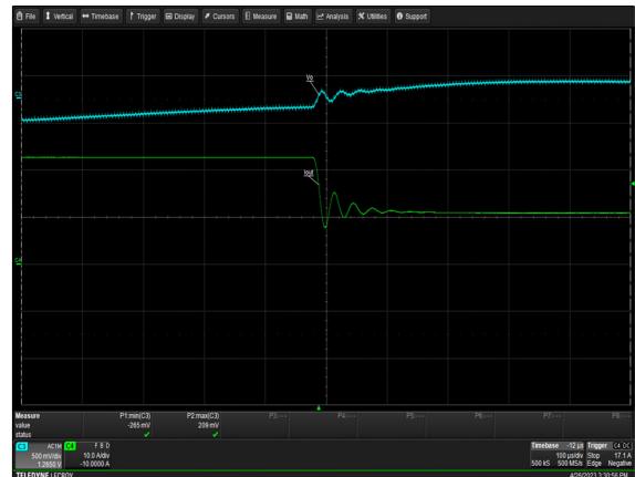
Figure 22: LCC1200-48U-9P Transient Response - Vo Deviation 100% to 50% load change (1KHz) 1A/uS slew rate Vin = 230Vac Ch 1: V O Ch 2: I O
