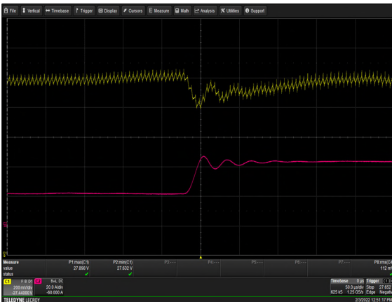
Figure 9: LCC1200-28U-9P Transient Response - V_o Deviation 50% to 100% load change (1KHz) 1A/ \mu s slew rate V_{in} = 230V_{ac} Ch 1: V_o Ch 2: I_o
