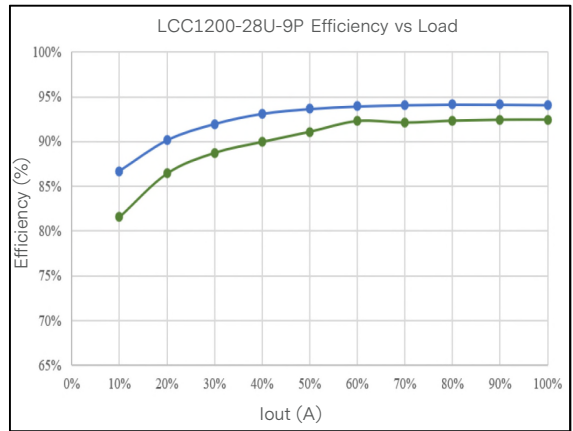
Figure 12: LCC1200-28U-9P Efficiency Curve @ 25°C Loading: I_{o\_main} = 10\%I_{o\_max} increment to full load
