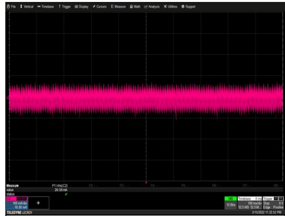
Figure 11: LCM4000HV-T Ripple and Noise Measurement
