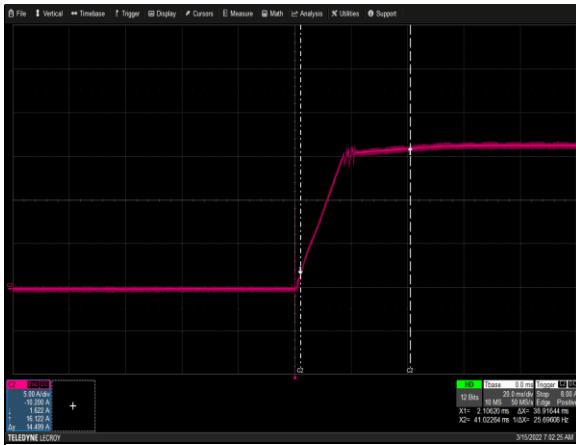
Figure 10: LCM4000HV-T Output Startup Characteristic
