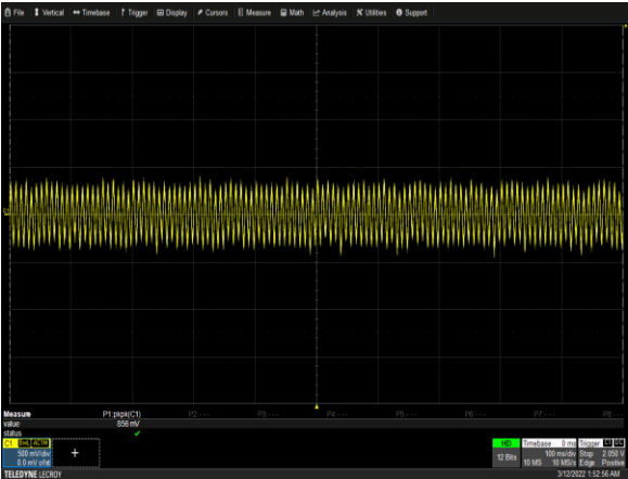
Figure 6: LCM4000HV-T Ripple and Noise Measurement Vin = 380VAC Load: Io = 16A Ch 1: Vo
