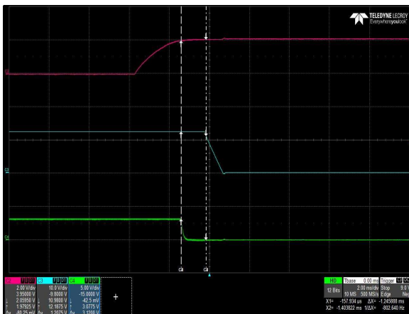
Figure 9: CSU2000AP-3-100 Turn Off Characteristic via PS_ON Load: I_o = 163.9A I_{SB} = 3.5A Ch 2: PS_ON Ch 3: V_O Ch 4: PWOK
