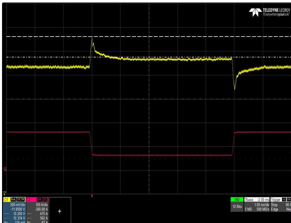
Figure 11: CSU2000AP-3-100 Transient Response - V_O Deviation 100% to 40% load change 0.5A/\mu s slew rate V_{in} = 230V_{ac} Ch 1: V_O Ch 2: I_o
