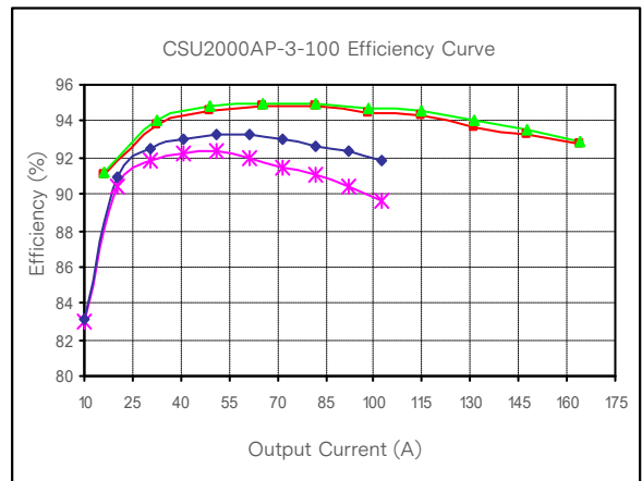
Figure 12: CSU2000AP-3-100 Efficiency Curve @ 25°C Loading: I_{o\_main} = 10\%I_{o\_max} increment to I_{o\_max}
