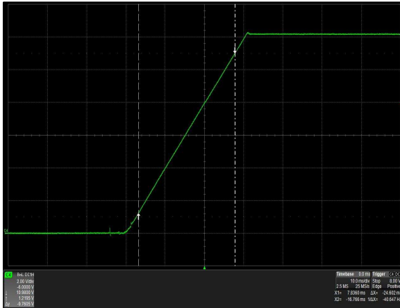
Figure 7: CSU2000AP-3-100 Output Voltage Startup Characteristic V_{in} = 90V_{ac} Load: I_o = 102.5A Ch 4: V_O
