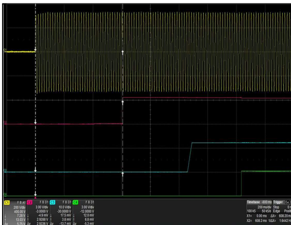
Figure 29: CSU2000AP-3-200 V_{IN\_GOOD} Assert Characteristic
