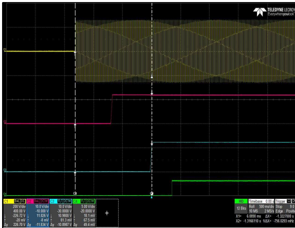
Figure 25: CSU2000AP-3-200 Turn-On Delay via AC Mains
