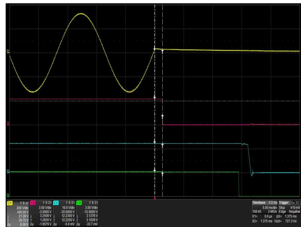
Figure 30: CSU2000AP-3-200 V_{IN\_GOOD} De-assert Characteristic
