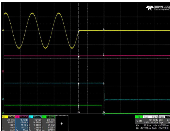
Figure 27: CSU2000AP-3-200 Hold-Up Time
