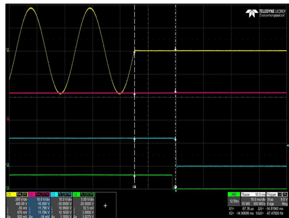
Figure 28: CSU2000AP-3-200 Hold-Up Time
