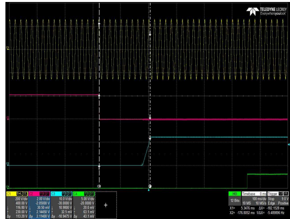
Figure 26: CSU2000AP-3-200 Turn-On Delay via PSON
